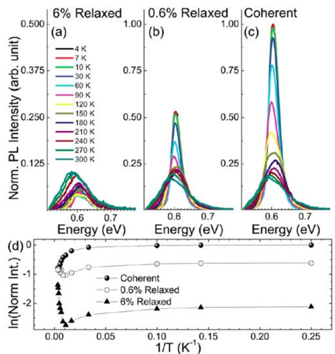
Fig. 1 Photoluminescence (PL) spectra as a function of the temperature for Ge 0.91 Sn 0.09 layers epitaxially grown on Ge-buffered Si(001) substrates.
