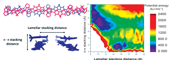
Fig. 15: Structure and calculated potential energy surface (PES) for C-PCPDTBT. The step size is 0.25 Å for the \pi - \pi stacking and 0.5 Å for the lamellar stacking.
