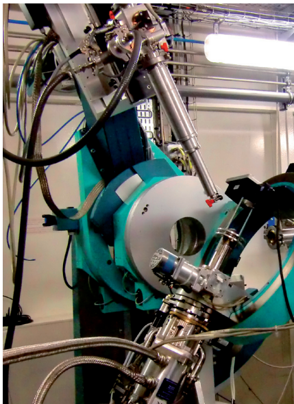
Fig. 4: The XMaS diffractometer supporting the sample cryostat and rotating magnet during the experiment.
