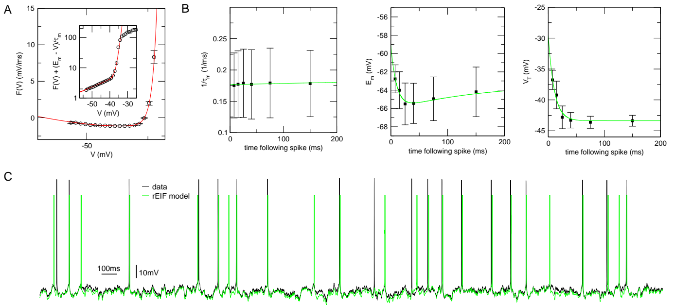
Fig. 4 Application of the dynamic I-V method with conductance injection. (A) The function F(V) = -I_{dyn}(V)/C is plotted (symbols) together with the fit (red) to the function (14). Inset: Two exponential components are clearly seen in a semi-log plot of F(V) with the leak currents subtracted. (B) Post-spike dynamics of the EIF model parameters (symbols) together with the fits to an exponential model. The time-dependent resting potential shows a clear biphasic response as was seen for layer-5 pyramidal cells in the current-injection protocol. (C) Comparison of the prediction of the rEIF model (green) with experimental data again shows good agreement in the subthreshold region and in the prediction of spike times.
