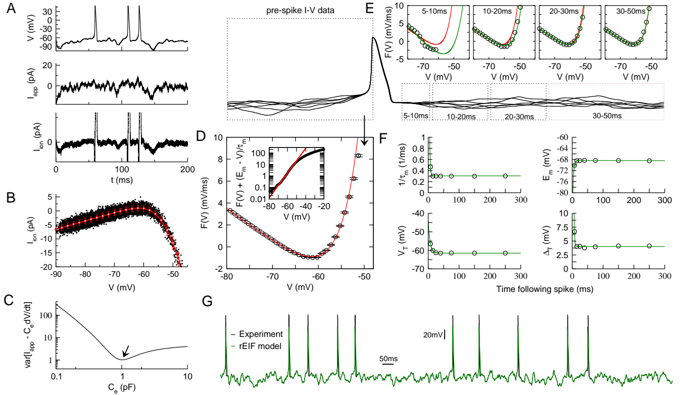
Fig. 1 Summary of the dynamic I-V curve method and its application to the Wang-Buzsáki model. (A) The derivative of the membrane voltage (top graph), multiplied by the cellular capacitance, is subtracted from the injected current (middle graph) to yield the intrinsic membrane current I_{ion} (bottom graph). (B) The intrinsic membrane current I_{ion} is plotted against the membrane voltage (black symbols). The dynamic I-V curve (red symbols) is obtained by averaging I_{ion} in small voltage bins. Error bars represent the standard deviation. (C) Measuring the cellular capacitance. At a fixed subthreshold voltage, the dynamic membrane current I_{ion} = I_{in} - CdV/dt has a variance that depends on the value of C used in the calculation; the correct value of C corresponds to the point of minimal variance. (D) Relating dynamic I-V curves and nonlinear integrate-and-fire models. The function F(V) = -I_{dyn}(V)/C (symbols) is plotted as a function of voltage, together with the EIF model fit (red line). Inset: semi-log plot of F(V) with leak current subtracted, showing a nearly exponential run-up. (E) Spike-triggered dynamic I-V curves. The functions F(V) measured in small time slices after each spike (symbols) are plotted together with the EIF fit (green) and the pre-spike I-V curve as a reference (red). At early times it is clearly seen that both the conductance and the spike threshold are significantly increased. (F) Dynamics of the EIF model parameters during the refractory period. The parameters obtained from the fits of the I-V curves in E are plotted as a function of the time since the last spike (symbols) and fitted with exponential functions (green). (G) Comparison of the prediction of the refractory EIF (rEIF) model (green) with a voltage trace of the Wang-Buzsáki model (black) shows excellent agreement, with 96% of the spikes correctly predicted by the EIF model within a 5ms window.
