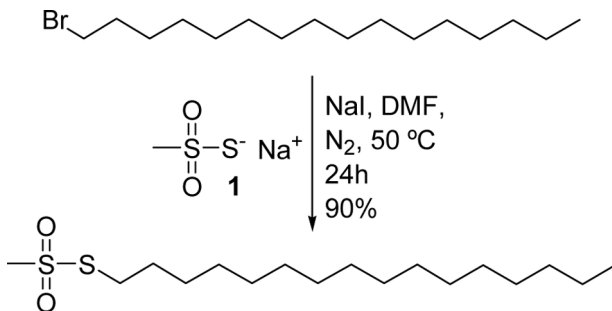
Scheme 1. Preparation of methanethiosulfonate lipid.
