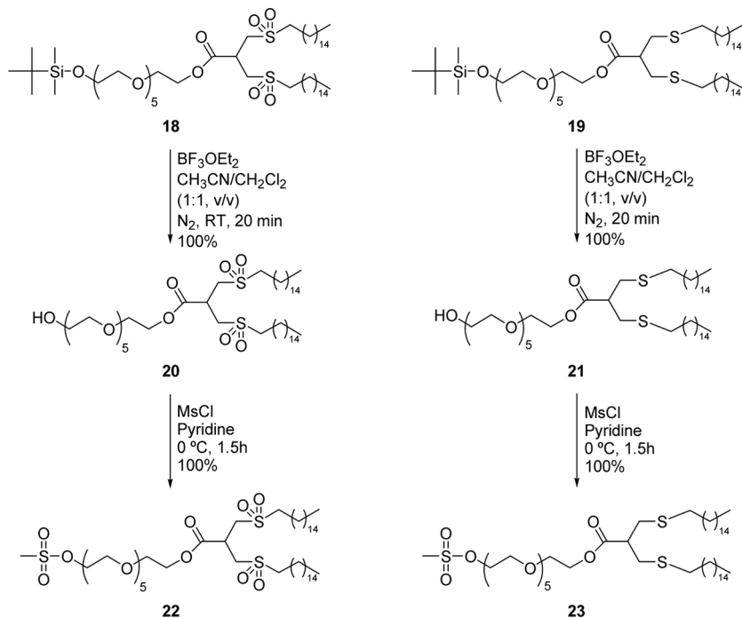
Scheme 8. Synthesis of the mesylated derivatives.
