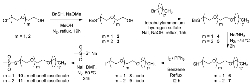
Scheme 2. Synthesis of two different single methanethiosulfonate chains.
