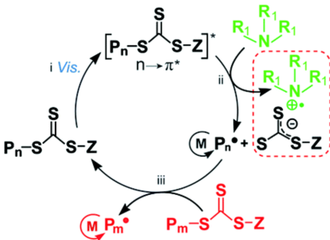
Scheme 2- showing the cycle of raft polymerisation present, and that it is still possible after the deoxygenation step.
