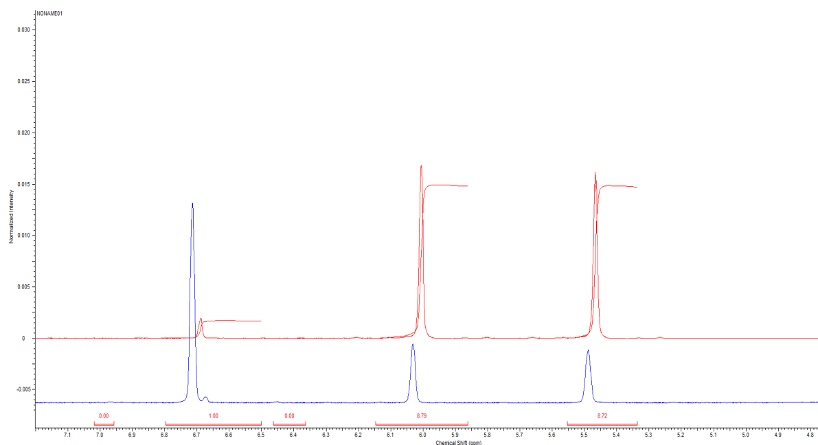
Figure 7- A ^1\text{H} NMR showing the difference in before the reaction (blue) and after reaction (red). Far left peak is that of mesitylene, the concentration of which does not change. The other 2 peaks are the vinyl peaks, corresponding to the double bond that has to be broken to form a polymer.
