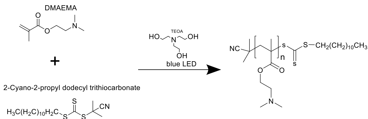
Scheme 3 – showing the polymerisation scheme for the formation of PDMAEMA
