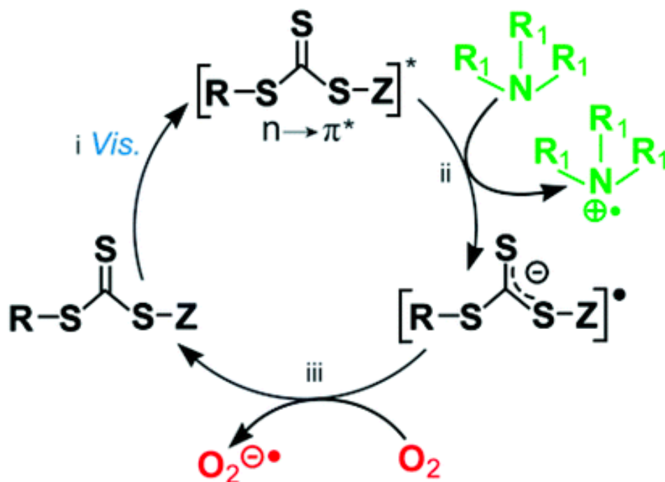
Scheme 1 – showing the proposed cycle for the deoxygenation that the TTC and tertiary amine provide. 17
