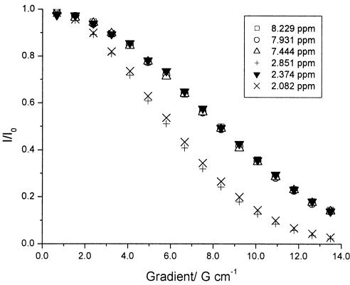
Figure 10: I/I_0 vs. G obtained from DOSY experiments on Co(II)(dmg) 2 .py.
