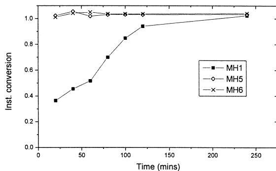
Figure 5: Instantaneous conversion versus time graph for emulsion polymerisations MH1, MH5 and MH6.
