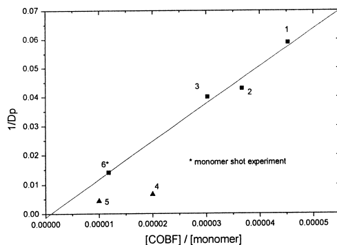
Figure 6: Pseudo Mayo plot for MMA/HEMA (70:30 molar ratio) emulsion copolymerisations using COBF as the transfer agent.
