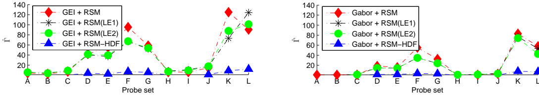
Fig. 7. Over the 12 probe sets on the USF dataset, the distribution of \hat{F} (i.e., the general ratio of false votes to true votes)
