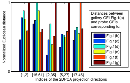
Fig. 4. Normalized Euclidean distances from gallery sample Fig. 1(a) to probe samples Fig.1(b)-Fig.1(g) based on different projection directions
