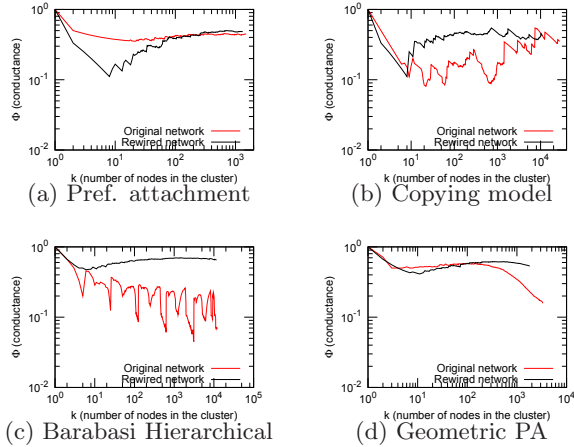
Figure 7: [Best viewed in color.] NCP for networks from commonly network generation models. Red curves are Local Spectral Algorithm on the original network, and black curves are Local Spectral Algorithm applied to a randomly rewired network.
