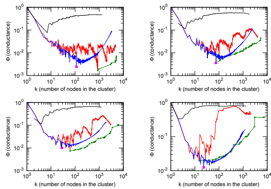
Figure 8: [Best viewed in color.] NCP plots for the Forest Fire Model at various parameter settings. The backward burning probability is p_b = 0.3 , and we increase (left to right, top to bottom) the forward burning probability p_f = \{0.26, 0.33, 0.35, 0.40\} . Note that the largest and smallest values for p_f lead to less realistic community profile plots.
