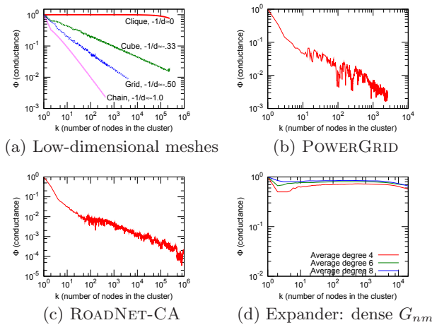
Figure 2: NCP plots for networks that “live” in low-dimensional spaces and for an expander-like graph.
