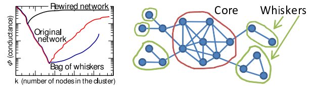
Figure 1: (a) Typical NCP plot. (b) Network structure as suggested by our experiments.
