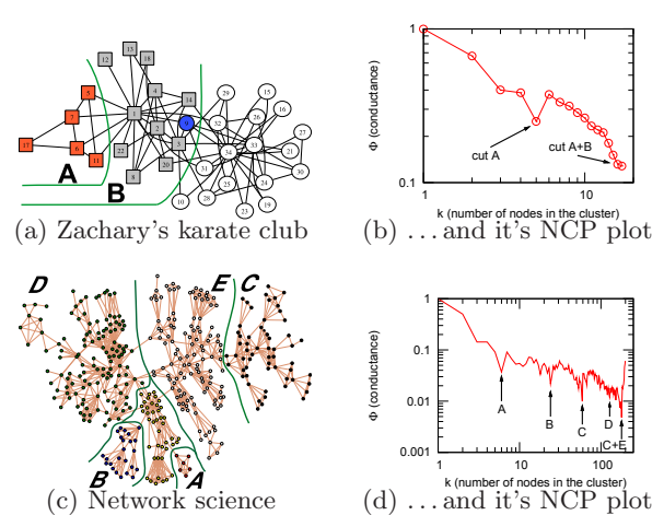
Figure 3: Depiction of several small social networks that are common test sets for community detection algorithms and their network NCP plots.
