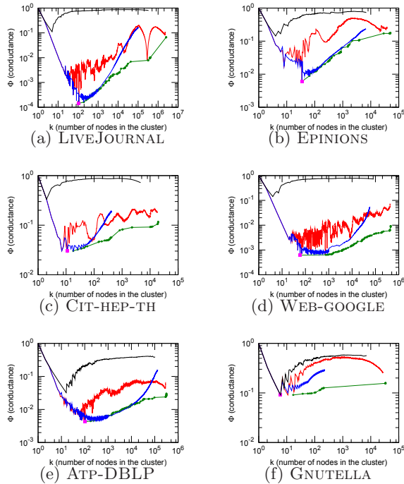
Figure 4: [Best viewed in color.] NCP plots for a representative sample of large networks. Red curves plot the Local Spectral Algorithm; green curves plot Metis+MQI; blue curves plot the Bag of Whiskers Heuristic; and black curves plot the Local Spectral Algorithm applied to a randomly rewired network.
