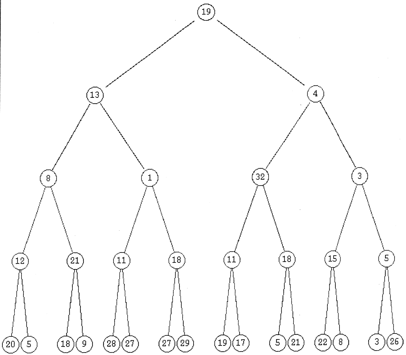
Figure 2: Heap representation for the array in Figure 1
