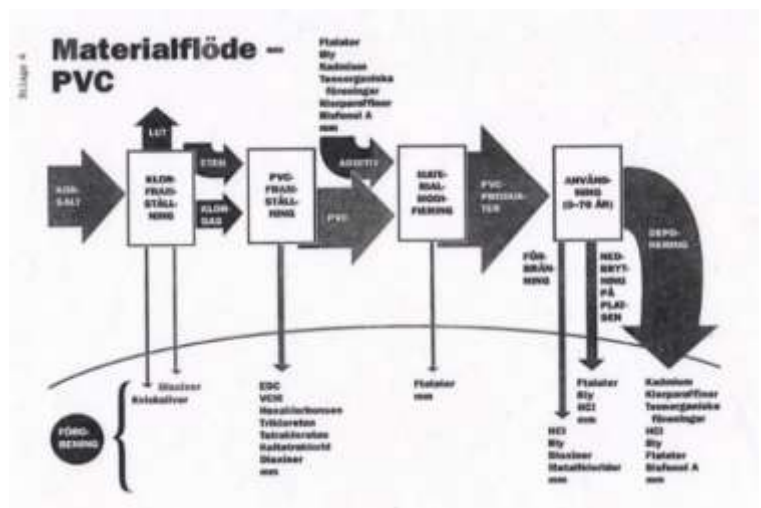
Flow chart for synthetic polymer PVC: very high energy content, and very high eco-impact factor
