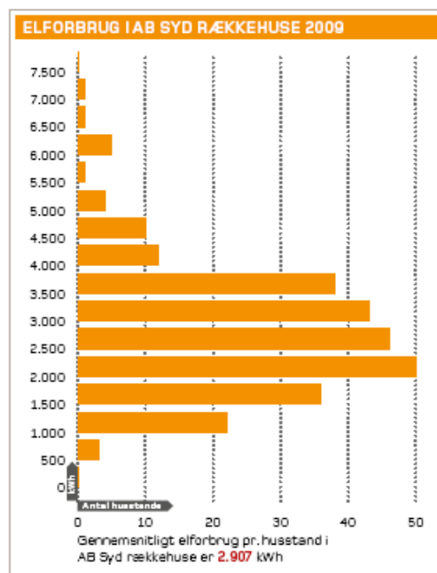
Electricity use variations in identical apartments, Albertslund, Denmark: the importance of behavioural issues
