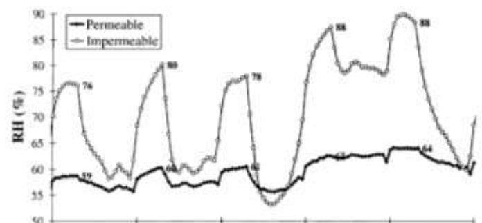
Hygroscopic materials: regulating indoor humidity
