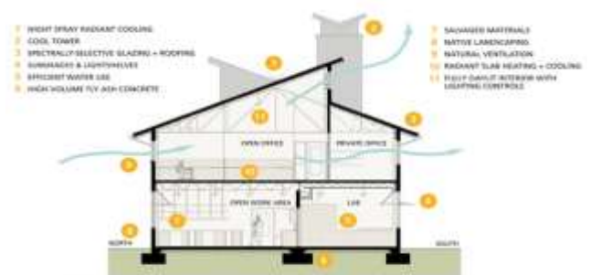
Enhanced stack effect ventilation, the Global Ecology Center, Washington
