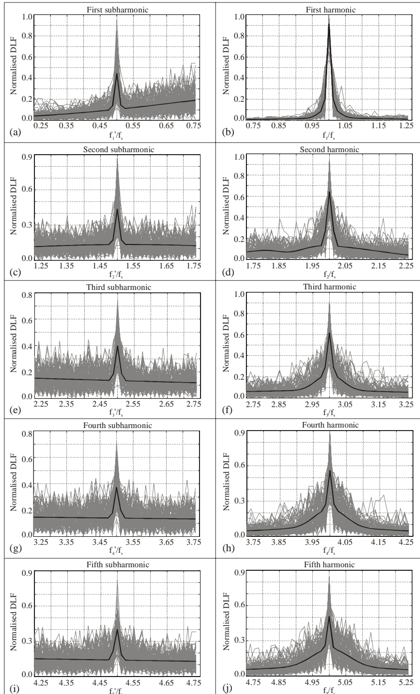
Figure 5: Normalised DLFs for the first five subharmonics (left column) and harmonics (right column).
