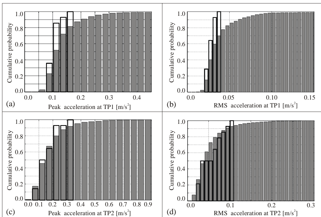
Figure 13: Cumulative probability for measured and simulated (a) peak acceleration at TP1, (b) RMS acceleration at TP1, (c) peak acceleration at TP2, and (d) RMS acceleration at TP2. Measured data are presented as solid lines while calculated responses are shown as grey.
