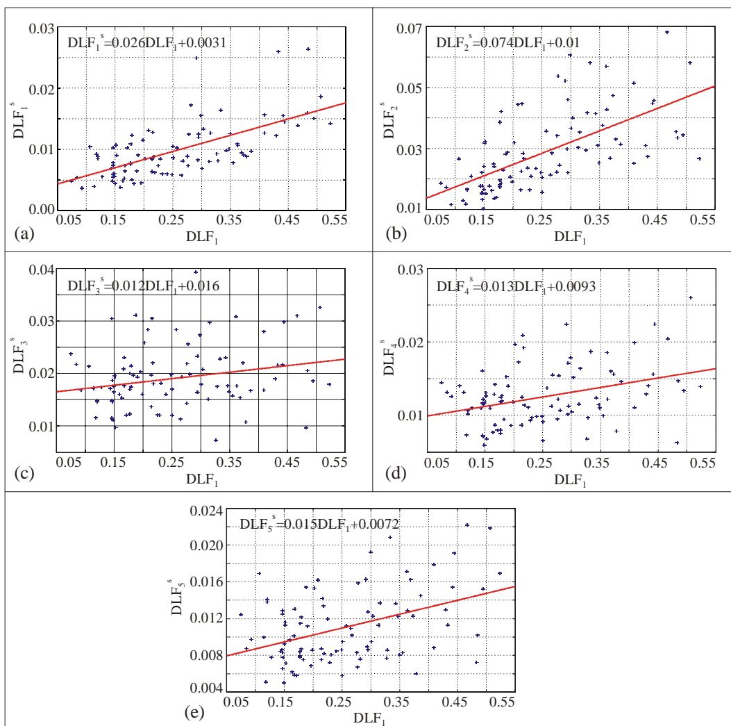
Figure 4: DLFs for subharmonics as functions of DLF_1 .
