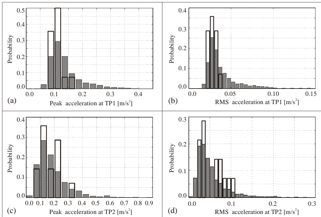
Figure 12: Probability of certain acceleration level for (a) peak acceleration at TP1, (b) RMS acceleration at TP1, (c) peak acceleration at TP2, and (d) RMS acceleration at TP2. Measured data are presented as solid lines while calculated responses are shown as grey.
