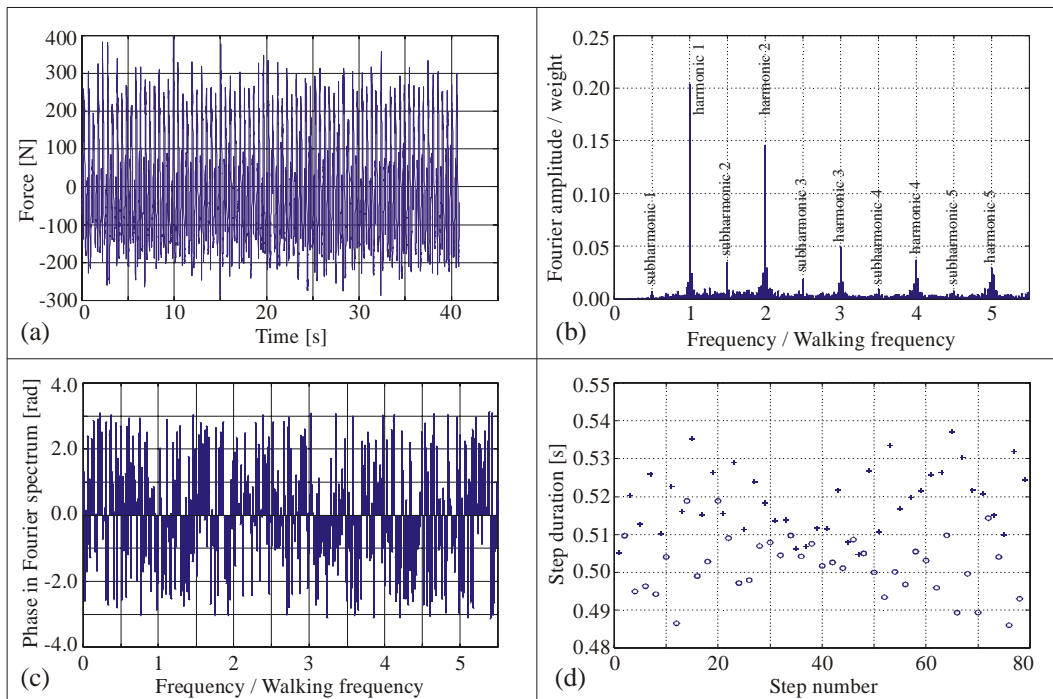
Figure 1: (a) Dynamic part of a force induced by walking. (b) Amplitude of force Fourier spectrum. (c) Phase of force Fourier spectrum. (d) Period of each step.
