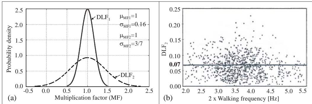
Figure 3: (a) Probability density function for multiplication factor for DLF 1 (solid line) and DLF 2 (dashed line). (b) DLF 2 measured by Kerr [9].
