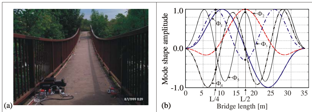
Figure 10: (a) Catenary footbridge. (b) Mode shapes for five vertical vibration modes.
