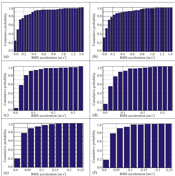
Figure 8: Cumulative probability that the RMS acceleration level for the whole response signal is smaller than or equal to the RMS acceleration level shown on the horizontal axis for the response in (a) Mode 1 due to measured forces, (b) Mode 1 due to simulated forces, (c) Mode 2 due to measured forces, (d) Mode 2 due to simulated forces, (e) Mode 3 due to measured forces and (f) Mode 3 due to simulated forces.
