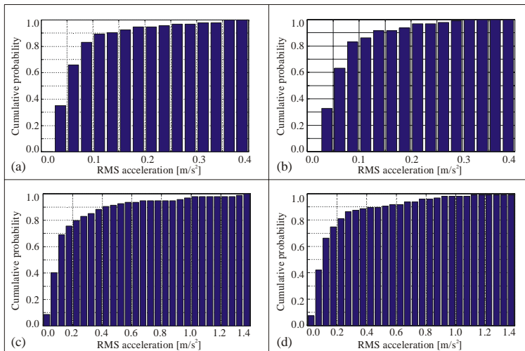
Figure 9: Cumulative probability of RMS acceleration response in Modes 2 and 3 due to (a) measured forces, (b) simulated forces. Cumulative probability of (c) total RMS response to measured forces, (d) total RMS response to simulated forces.
