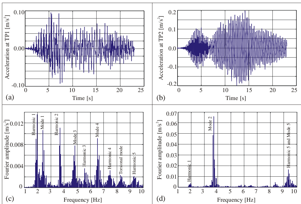
Figure 11: Measured time history at (a) TP1 and (b) TP2. Fourier spectrum of signal at (c) TP1 and (d) TP2.
