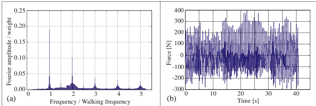
Figure 7: (a) Force spectrum for force shown in Fig. 1(a) according to the force model adopted. (b) Force reconstructed in the time domain.
