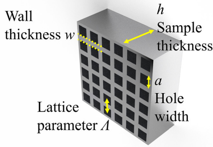
FIG. 1. (Color online) Schematic diagram of a holey metamaterial defined by \Lambda , a , w , and h .
