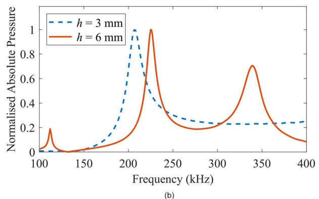
FIG. 3. (Color online) (a) Geometry of the 3D single-channel model showing the incident wave direction. (b) The simulated absolute value of pressure for h = 3 mm and h = 6 mm, showing clear FP peaks.
