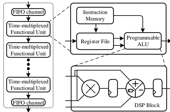
Fig. 2: A programmable processing pipeline.
