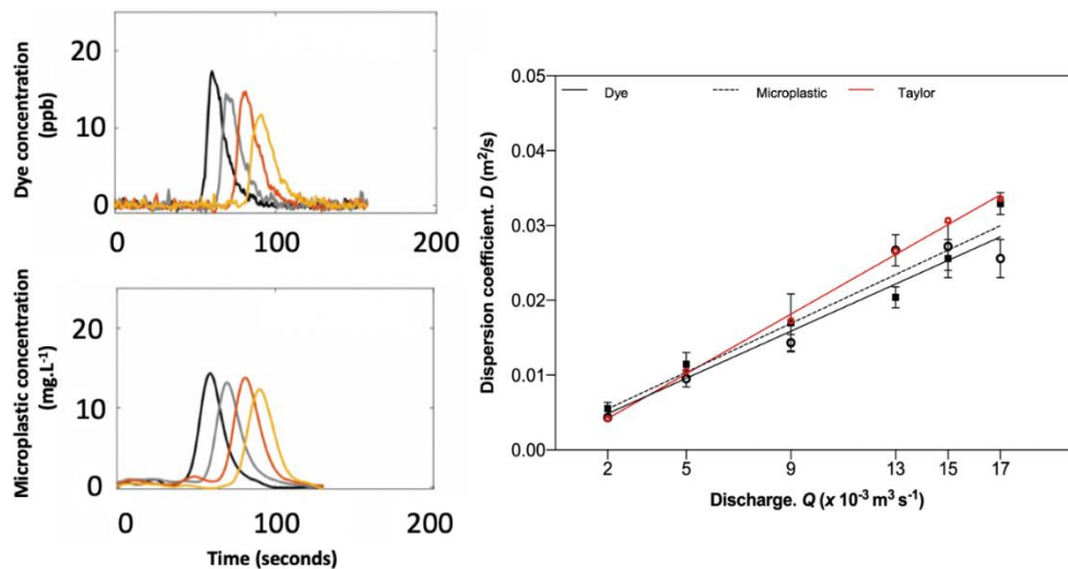
Figure 1: Longitudinal Dispersion in uniform open channel flow of a solute tracer and microplastics compared to Taylors (1953, 1954) classical theory (adapted from Cook et al. (2020)).
