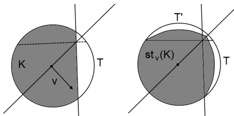
Figure 7: st_v(K) contains less of the boundary of B_\sigma(0) than K .
