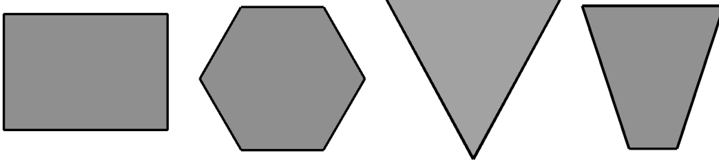
Figure 3: A few hyperplane cross-sections of Q_3 (not to scale) corresponding to the planes \{x : \langle x, v \rangle = a\} where v and a are (from left to right): v = (1, 1, 0) , a = 0 ; v = (1, 1, 1) , a = 0 ; v = (1, 1, 1) , a = 0.5 and v = (1, 1, 0.5) , a = 0.5 .
