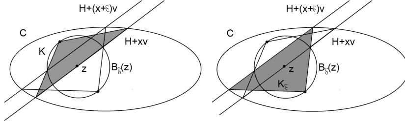
Figure 1: Constructing “conical caps”.
