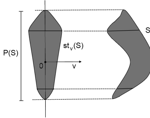
Figure 5: Steiner symmetrization.
