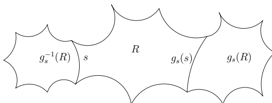
Figure 6.1: Side-pairings: g_s carries g_s^{-1}R to R and s to g_s(s) .
