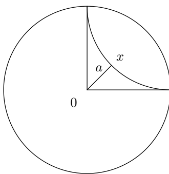
Figure 2.18: Computing Schweikart's constant.
