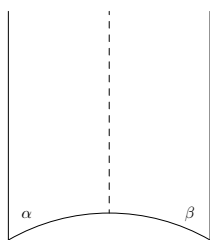
Figure 2.22: Area of a triangle with angles \alpha, \beta, 0 .
