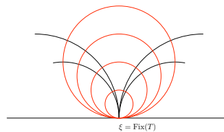
Figure 3.12: Action of a parabolic in general position.
