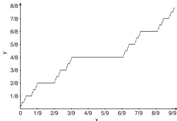
Fig. 1. The graph of the Cantor function G . This graph is sometimes called “Devil’s staircase”.
