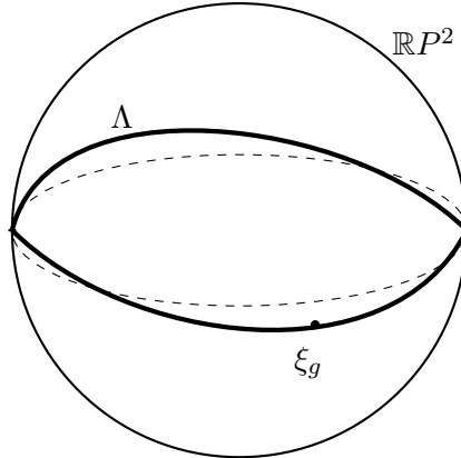
FIGURE 1. Here \rho is a representation into \mathrm{SL}(3, \mathbb{R}) and \Lambda \subset \mathbb{R}P^2 is the associated limit set. For g \in \Gamma \setminus \{1\} , the point \xi_g is an attracting fixed point for \widehat{\rho}(g) : \mathbb{R}P^2 \rightarrow \mathbb{R}P^2 .
