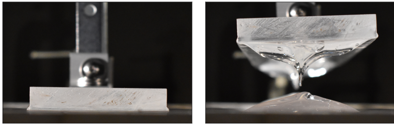
Figure 14: Photographs of lift-off experiments with Carbopol showing the effects of adhesion.
