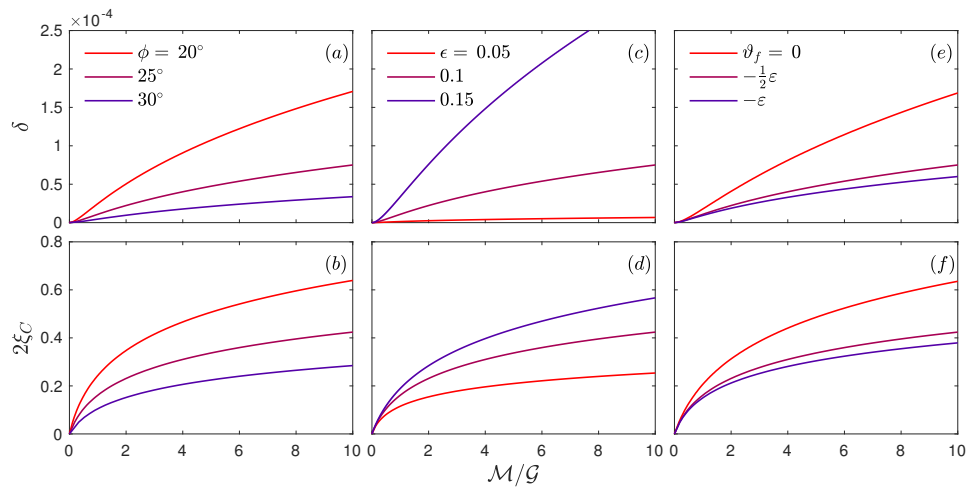
Figure 5: Penetration depth, \delta , and contact length, 2\xi_C , against non-dimensional load M/G for (a–b) \phi = 20, 25, 30^\circ , (c–d) \epsilon = 0.05, 0.1, 0.15 , and (e–f) \vartheta_f = -[0, \frac{1}{2}, 1] \times (\frac{1}{4}\pi + \frac{1}{2}\phi) . Aside from those choices, the parameters are \epsilon = 0.1 , \vartheta_f = -\frac{1}{2}(\frac{1}{4}\pi + \frac{1}{2}\phi) and \phi = 25^\circ .
