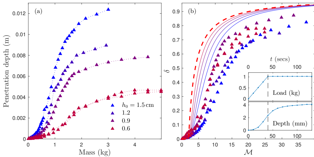
Figure 8: Indentations of the plate into Carbopol layers of different depth h_0 , with penetration depths plotted as in figure 7. In (b), the dashed line with \delta = 1 - 2/M shows the \mathcal{G}/\mathcal{M} \rightarrow 0 limit. The inset plots an additional experiment where the load is increased up to 1 kg then held fixed.
