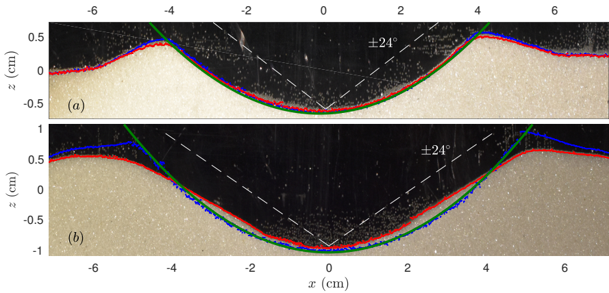
Figure 15: Profiles of the ballotini surface before (blue) and after (red) the lift-off of the cylinder. (a) Shallower indentation with minor surface motion generated by lift-off. (b) Deeper indentation, with significant inward avalanching occurring due to lift-off. D = 0.1 mm. The green line indicates the position of the cylinder before lift-off. The white dashed lines show the angle of friction \phi .
