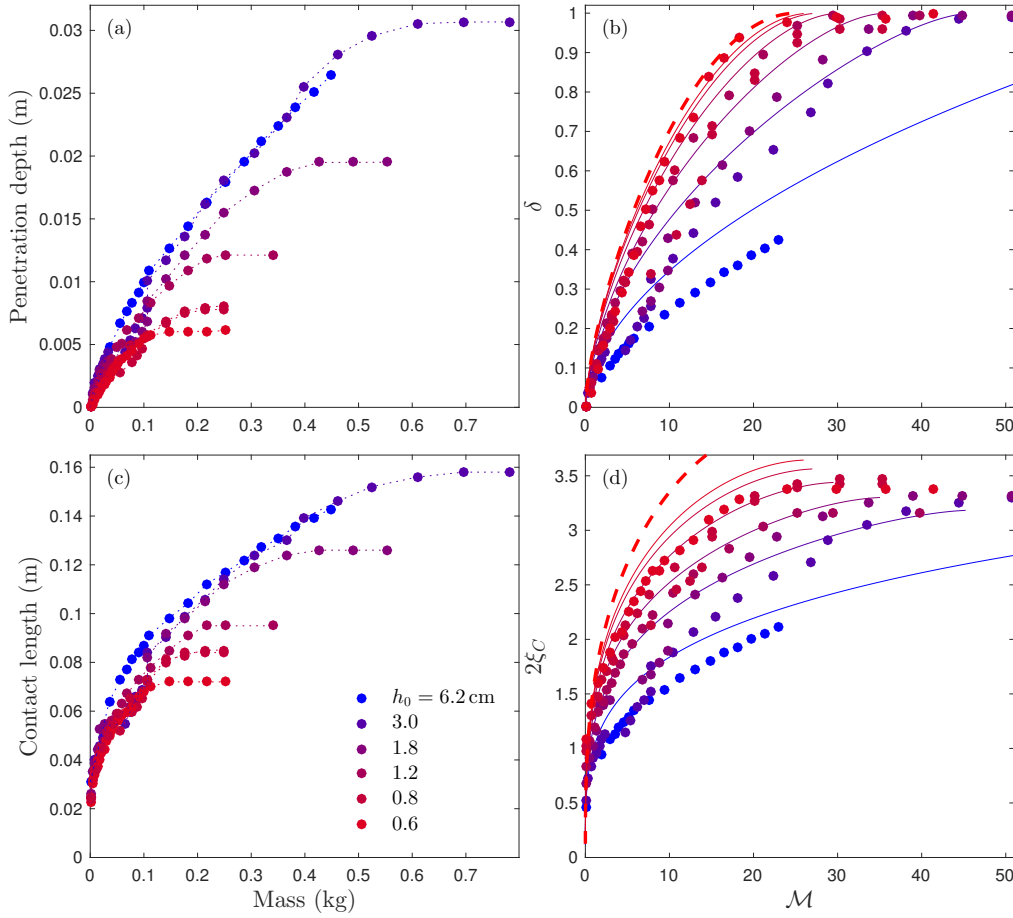
Figure 16: Indentations of the sphere into Carbopol layers of different depth h_0 , with data plotted as in figure 7. In (b) and (d), the dashed line shows the \mathcal{G}/\mathcal{M} \rightarrow 0 limit, \xi_C \rightarrow 2\sqrt{\delta} and (A 3).
