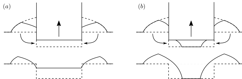
Figure 13: Lift-off mechanisms: (a) reverse squeeze flow, (b) avalanching.
