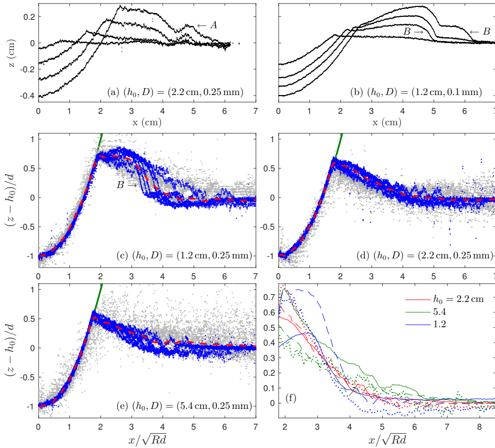
Figure 11: (a)-(b) Ballotini surface profiles for the layer depths h_0 and particle diameters D indicated. (c-e) show scaled profiles for the (h_0, D) combinations indicated, with the seven deepest penetrations in darker blue and ten shallower penetrations in light gray. The dashed lines show the averages of the data and the green solid lines indicate the cylinder. (f) plots the averaged scaled profiles, with the different layer depths colour coded as indicated and the particle diameters D = 0.1\text{mm} (solid), 0.25\text{mm} (dashed) and 0.5\text{mm} (dotted). Features marked A denote optical distortions through the cylinder; B denotes a genuine sharp variation in the surface.
