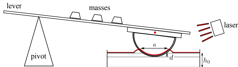
Figure 6: Sketch of the experimental set-up.
