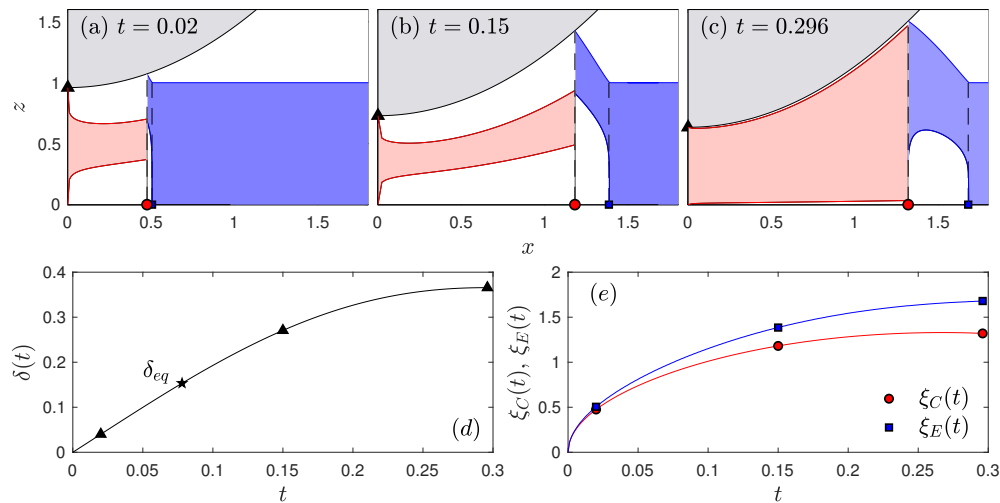
Figure 4: (a)–(c) Numerical solution for a cylinder dropped onto a Herschel Bulkley substrate with n = \frac{1}{3} , with \dot{\delta}_0 = 2 and \mathcal{M} = \mathcal{G} = \mathcal{V} = 1 , showing three snapshots of the flow patterns. Indicated are the edge of cylinder (black), the free surface (blue), the yield surfaces in the squeeze flow (red) and free surface flow (blue); the contact line and flow front are marked by vertical dashed lines. The cylinder and plug flows are shaded. Below are time series of (d) \delta(t) and (e) contact length and flow front; the triangles indicate the times of the snapshots in (a)–(e) and the star in (d) is the equilibrium depth \delta_{eq} of see §3(f).
