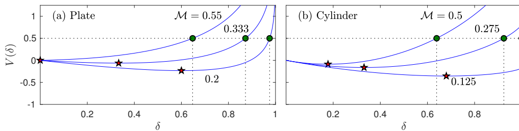
Figure 12: Potential functions V(\delta) for (a) the plate and (b) the cylinder for three values of \mathcal{M} indicated. The stars show \delta_{eq} ; the dots indicate \delta_f assuming that \dot{\delta}_0 = 1 . For the plate, \delta_{eq} = 0 if \mathcal{M} < 2 (but the plate still penetrates to \delta_f > 0 for \dot{\delta}_0 > 0 ) and contact cannot be established with the underlying surface \delta_f < 1 . For the cylinder, contact is possible when \frac{1}{2}\dot{\delta}_0^2 > V(1) .
