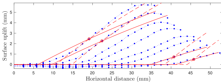
Figure 9: Profiles of the free surface deformation in Carbopol for the cylinder with h_0 = 1.2 cm. The theoretical predictions in (5.1) and (5.2), pinned at the points indicated by the circles, are plotted as solid or dashed lines (respectively).
