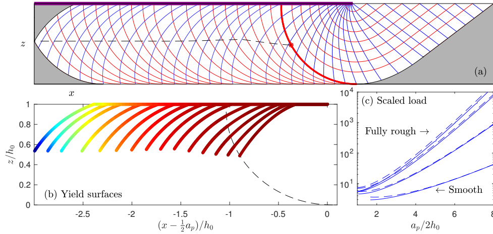
Figure 3: (a) Sliplines for a Mohr-Coulomb layer with a = 9.2h_0 , \phi = 24^\circ and \vartheta_f = -\frac{2}{3}(\frac{1}{4}\pi + \frac{1}{2}\phi) . The dashed line shows the locus of the points where \vartheta = 0 . In (b), the upper yield surfaces are shown for various a , coloured according to the local vertical force density with the overlying weight of plugged material subtracted, and with the last self-similar \alpha -line shown by the dashed line. In (c) we plot the load scaled by \frac{1}{2}\rho g a^2 W (the Terzaghi coefficient) for \theta_f = -[0, \frac{1}{3}, \frac{2}{3}, 1] \times (\frac{1}{4}\pi + \frac{1}{2}\phi) . The dashed lines show the asymptotic prediction for a \gg h_0 in §4.
