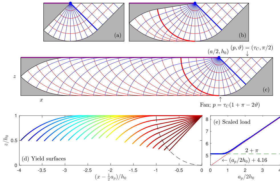
Figure 2: Sliplines for a cohesive layer, showing (a) the Prandtl solution for which the fan first touches the base ( a = \sqrt{2}h_0 ), and (b)–(c) longer indenters in which the fan widens up to an angle of 3\pi/4 and the slipline pattern is continued to the left ( \alpha -lines shown in red and \beta -lines in blue). The arc bounding the centred fan to the left (thicker red curve) is the \alpha -line from which the slipline field is constructed. (d) shows a selection of upper yield surfaces for varying a_p , coloured according to the local vertical force density; the dashed line shows the edge of the fan. (e) plots the load, scaled by aW\tau_Y , against \frac{1}{2}h_0^{-1}a_p , with the shallow and deep limits indicated.
