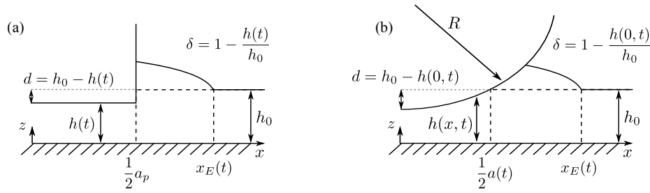
Figure 1: Sketches of the problem geometries: (a) a flat-based indenter or plate, and (b) the locally parabolic underside of a cylinder.
