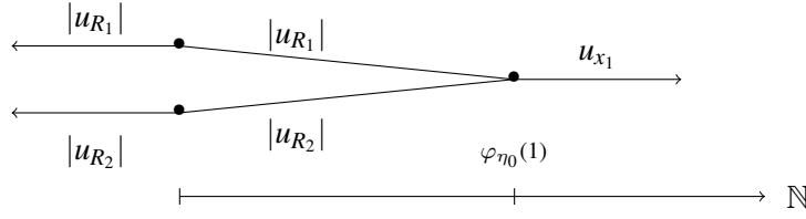
Figure 1: Tropical curve
