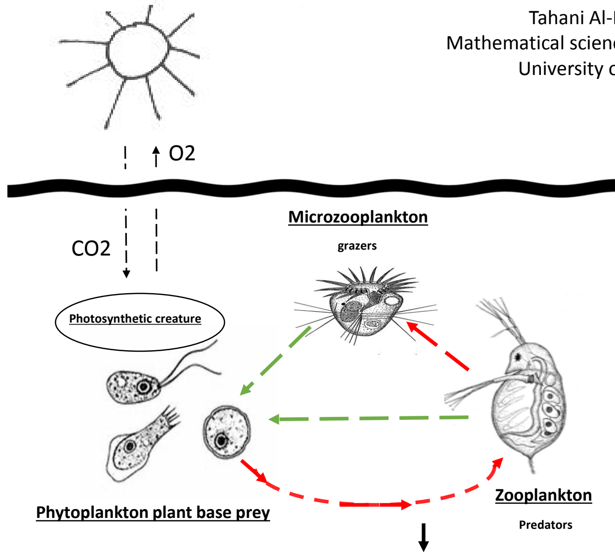
Infochemical release as a defense mechanism from Phytoplankton
