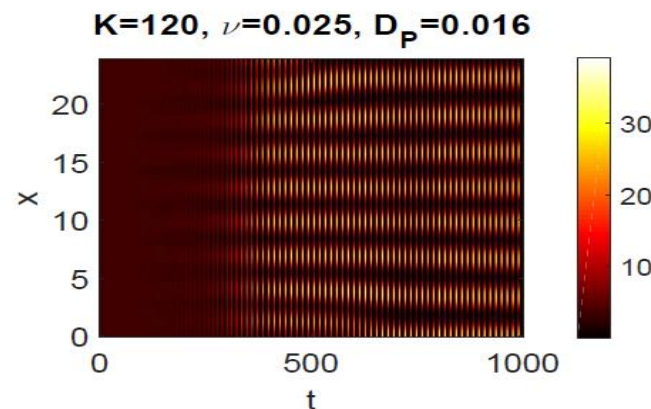
Numerical simulation of two trophic Plankton Model
