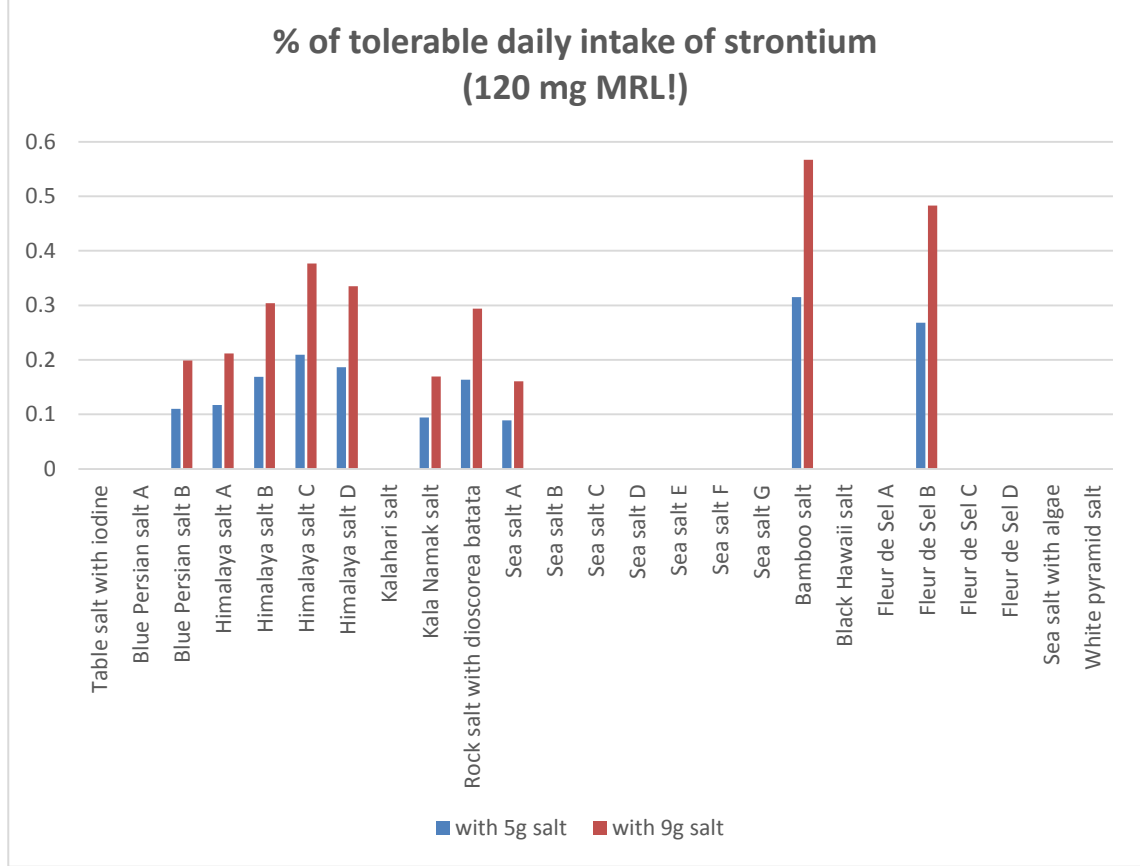
Figure 13: Strontium content in comparison with tolerable intake levels
