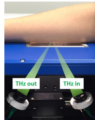
Fig. 1. Photograph of in vivo THz imaging set up to image the skin on the volar forearm.
