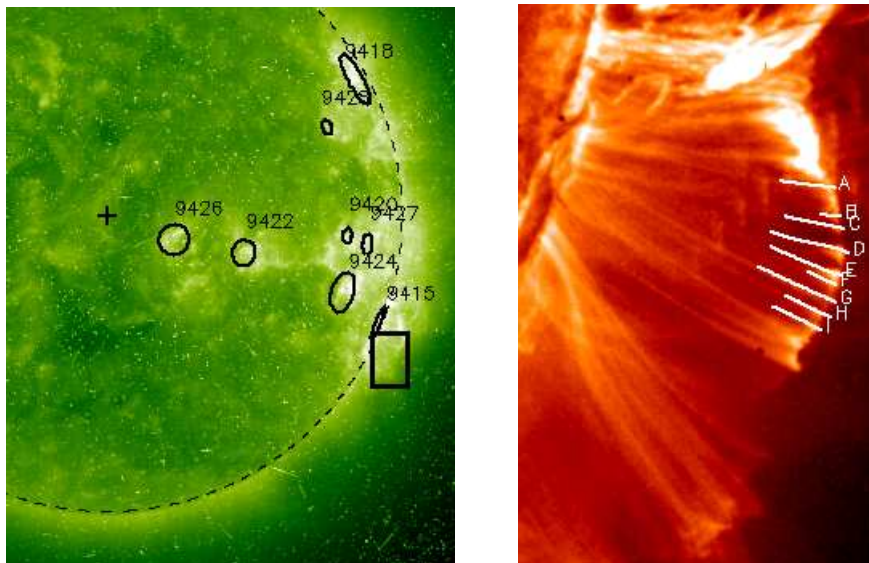
Figure 1. Left: Subfield of an 195 Å EIT/SoHO full-disk image on 15 April 2001 at 20:24 UT with NOAA active regions and field of view of the TRACE subfield. Right: Subfield of TRACE observation of the same day at 22:11 UT with paths used in the analysis.
