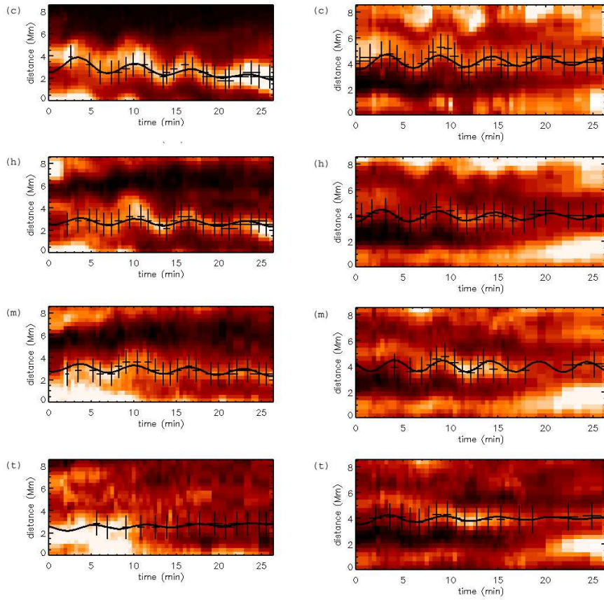
Figure 3. Left: Set of four images I_{D,x}(y, t) of the segments c,h,m and t, corresponding to x = 0.7, 3.6, 6.4 and 10.0 Mm from the loop top respectively, along the loop in path D. The displacement coordinates are shown as crosses. The solid curve is a fitted function of the form (1) with n=1 . Right: Same as before, but for path G. The segments c,h,m and t correspond to x = -0.1, 3.5, 7.1 and 10.6 Mm from the loop top respectively.
