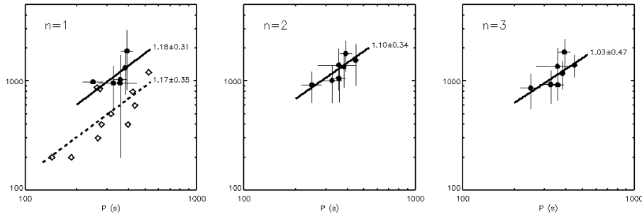
Figure 6. Plot of the measured decay times \tau with respect to the oscillation period P as solid circles for the cases n=1,2,3 . The diamond symbols show the measurements from (Nakariakov et al. , 1999) and (Aschwanden et al. , 2002) that were used by (Ofman, 2002) to deduce the powerlaw relationship \tau \sim P^{1.17 \pm 0.35} , here shown as a dashed line. The solid line is a best powerlaw fit of the measurements of this loop arcade. The value of the power index of each powerlaw fit is shown. The powerlaw fit for n=1 includes two outlying measurements from (Ofman, 2002). Without these no reasonable fit is possible for n=1 .
