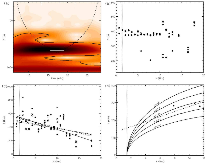
Figure 5. Overview of the period and amplitude of the loop oscillations in path D. (a): magnitude of the wavelet transform of the displacement coordinates of I_{D,x} at x = 11 Mm from the loop top. The white lines bracket the two detected periodic signatures at 240 and 400 s respectively. (b): measured oscillation periods as a function of distance x . The solid circles are the periods found with the wavelet analysis. The crosses, stars and diamonds are the periods derived by the curve fitting method with n=1,2 and 3 respectively. (c): Displacement amplitude A for the 400 s oscillation as a function of distance x . The crosses, stars and diamonds are the amplitudes derived by the curve fitting with n=1,2 and 3 respectively. The circles are the amplitudes found with the wavelet analysis. Each dataset is fitted by a straight line (solid: wavelet fit, dashed: n=1 , dot-dashed: n=2 , triple dot-dashed: n=3 ). (d): Displacement amplitude A for the 240 s oscillation. Only wavelet measurements are available and are shown as circles. The dashed line is a linear fit. The solid curves represent the profile of a second harmonic standing mode for several amplitude values. The dotted line in plots (b),(c) and (d) shows the position x_{\text{top}} of the loop top.
