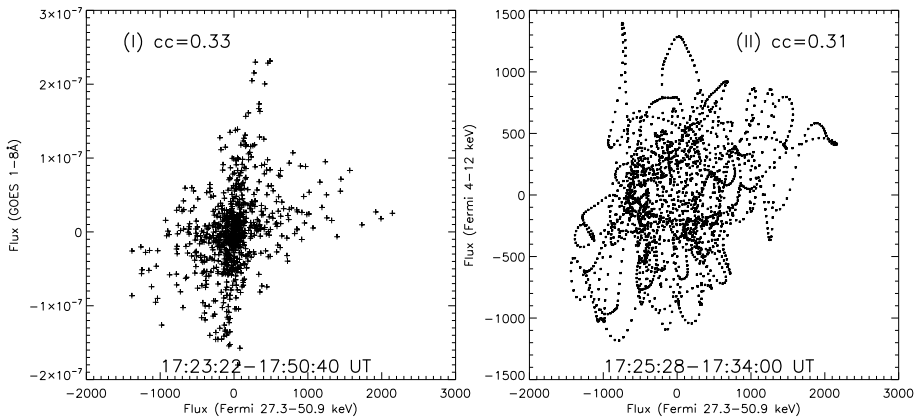
Figure 11 Correlation of the fast-varying components of GOES at 1–8 Å and of Fermi at 4–12 keV with those of Fermi at 27.3–50.9 keV. The correlation coefficients (cc) are given.
