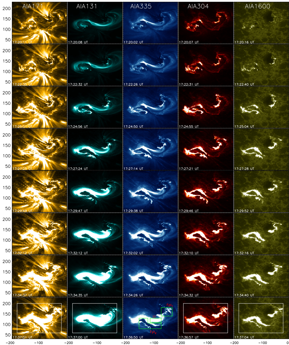
Figure 1 Time sequences of SDO/AIA maps at 171 Å, 131 Å, 335 Å, 304 Å, and 1600 Å between 17:20 UT and 17:37 UT. The flare loop footpoints (Fpt 1 and Fpt 2 ) and the loop top (Lt) are marked by three green boxes in the last AIA 335 image. The light curves in the white box are shown in Figure 4.
