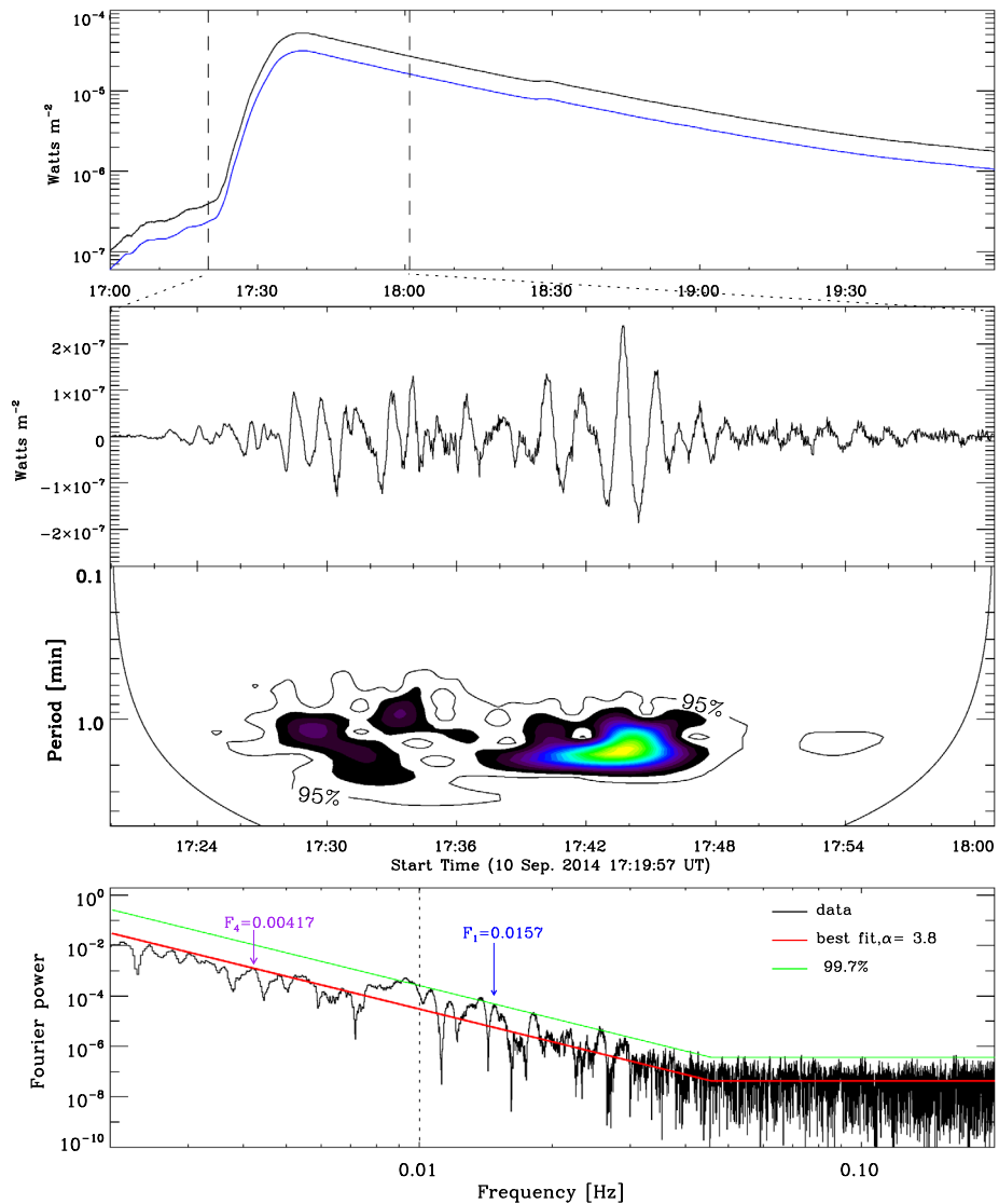
Figure 2 Upper panel: the light curve (black) of GOES SXR at 1–8 Å and its slowly varying component (blue, after multiplying by 0.6) for the 10 September 2014 solar flare. Second and third panels: the fast-varying component in the interval between the two vertical dashed lines (upper panel) and its wavelet spectrum. Bottom: Fourier power of the GOES light curve, with the vertical dotted line marking the position (at the frequency of 0.01 Hz) that separates the domains of the fast- and slowly varying components. The red solid line is the best fit, and the green line shows the confidence level at 99.7 %. Two frequencies of 0.0157 Hz (about one minute) and 0.00417 Hz (about four minutes) are marked by blue and purple arrows, respectively.
