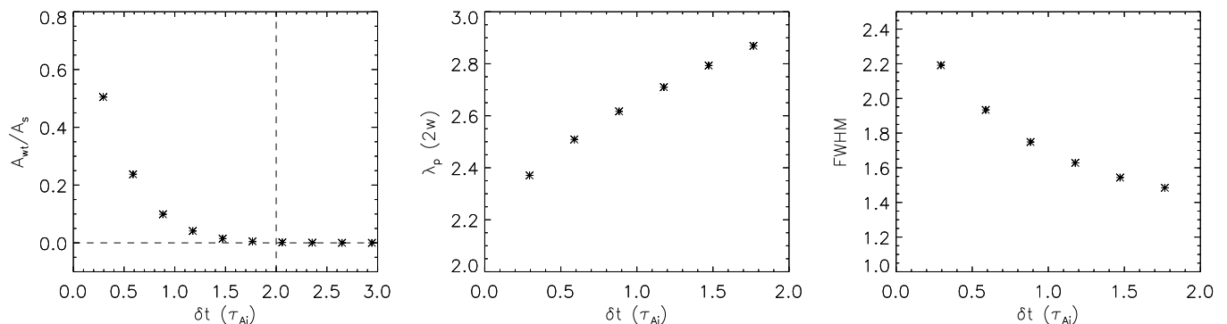
Fig. 4. Left: the amplitude ratio of the fast wave train and slow wave measured at t = 110 plotted against the driver duration in units of the Alfvén transit time across the waveguide. The cutoff above which the fast wave train is no longer considered to be efficiently excited is shown by the vertical dashed line. Middle: the wavelength of peak spectral amplitude (in units of the waveguide width) of the fast wave train plotted against the driver duration. Right: the spectral width of the fast wave train signal plotted against the driver duration.
