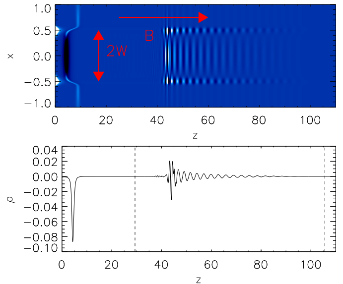
Fig. 2. Top: the perturbation to the equilibrium density at t = 110 from a driver with \delta t = 0.58 \tau_{Ai} . The slow wave can be seen at z \sim 10 and the fast wave train between z \sim 40 and z \sim 100 , both propagating to the right. The waveguide width is indicated by 2w , and the magnetic field direction by B . Bottom: the perturbation to the equilibrium density measured along the centre of the waveguide ( x = 0 ) from the above simulation output. The region between the dashed vertical lines denotes the section of the signal used for analysis of the fast wave train.
