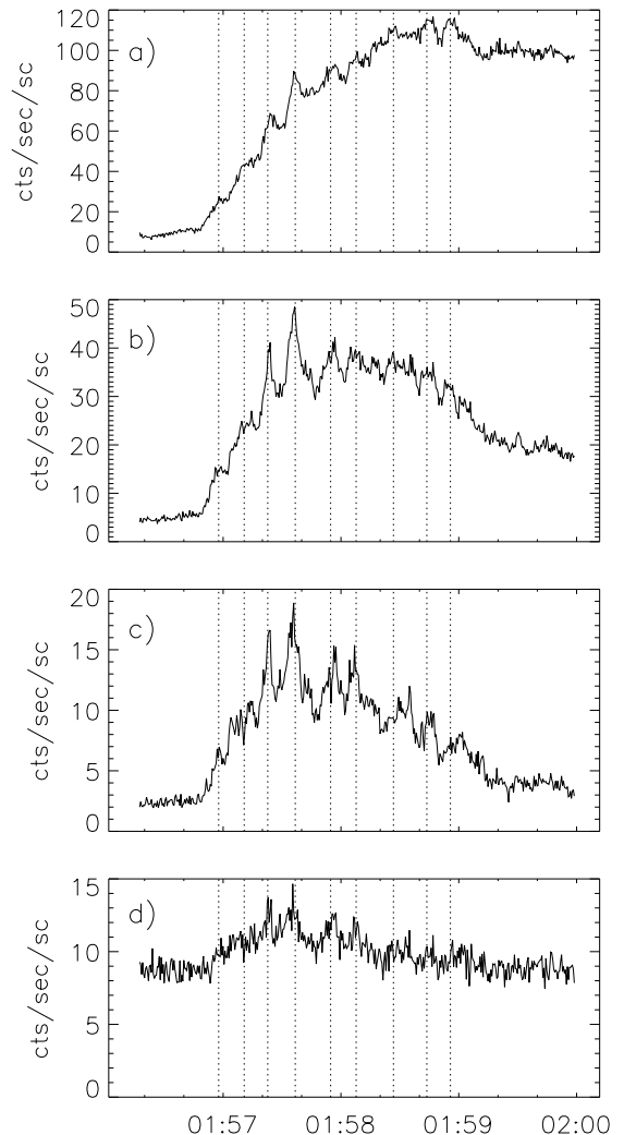
Fig. 2. Hard X-ray light curves from the Yohkoh satellite, observing the solar flare of 8th May 1998. a) : X-ray counts in the L (13 - 23 keV) range, b) : X-ray counts in the M1 (23 - 33 keV) range, c) : X-ray counts in the M2 (33 - 53 keV) range, d) : X-ray counts in the H (53 - 93 keV) range.
