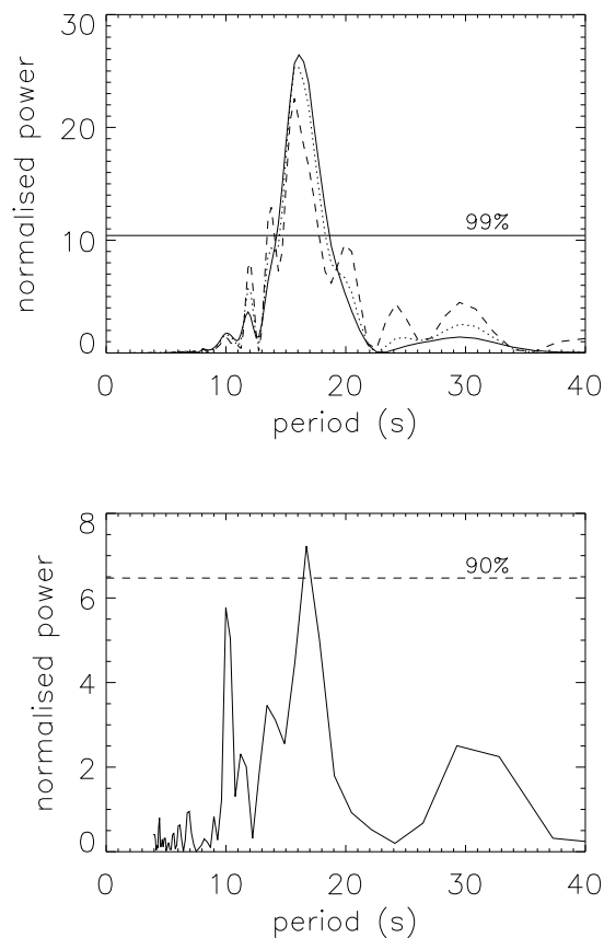
Fig. 3. Top panel: Lomb-Scargle periodogram (Scargle 1982) of the 17 GHz modulation depth from the Nobeyama Radioheliograph. Dashed line : periodogram without a window function; dotted line : periodogram using a Hann window function; solid line : periodogram using a Blackman-Harris window function. The periodogram reveals an oscillation period of 16 s, above the 99% confidence level. Bottom panel: Lomb-Scargle periodogram of the M1 (23-33 keV) X-ray modulation observed by the Yohkoh satellite.
