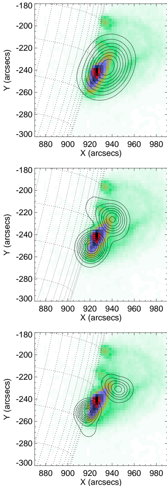
Fig. 5. Contour maps of hard X-ray emission overlaid on a soft X-ray image of the flaring loop at 01:57:50 UT, during the oscillatory phase. Top: the L (13 – 23 keV) channel, centre: the M1 (23 – 33 keV) channel, bottom: the M2 (33 – 53 keV) channel.
