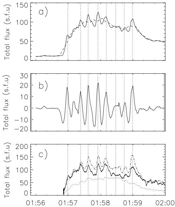
Fig. 1. a) : Integrated flux time profile of microwave emission at 17 GHz for the solar flare of 8th May 1998, as observed by NoRH. Overlaid with the dashed line is the background emission profile obtained via 20 s smoothing of the integrated flux signal. b) : The signal after subtraction of the background profile from the integrated flux. c) : Solar flux time profiles of microwave emission at 9.4 GHz (dot-dashed line), 17 GHz (solid line) and 3.75 GHz (dotted line), obtained by the Nobeyama Radiopolarimeters.
