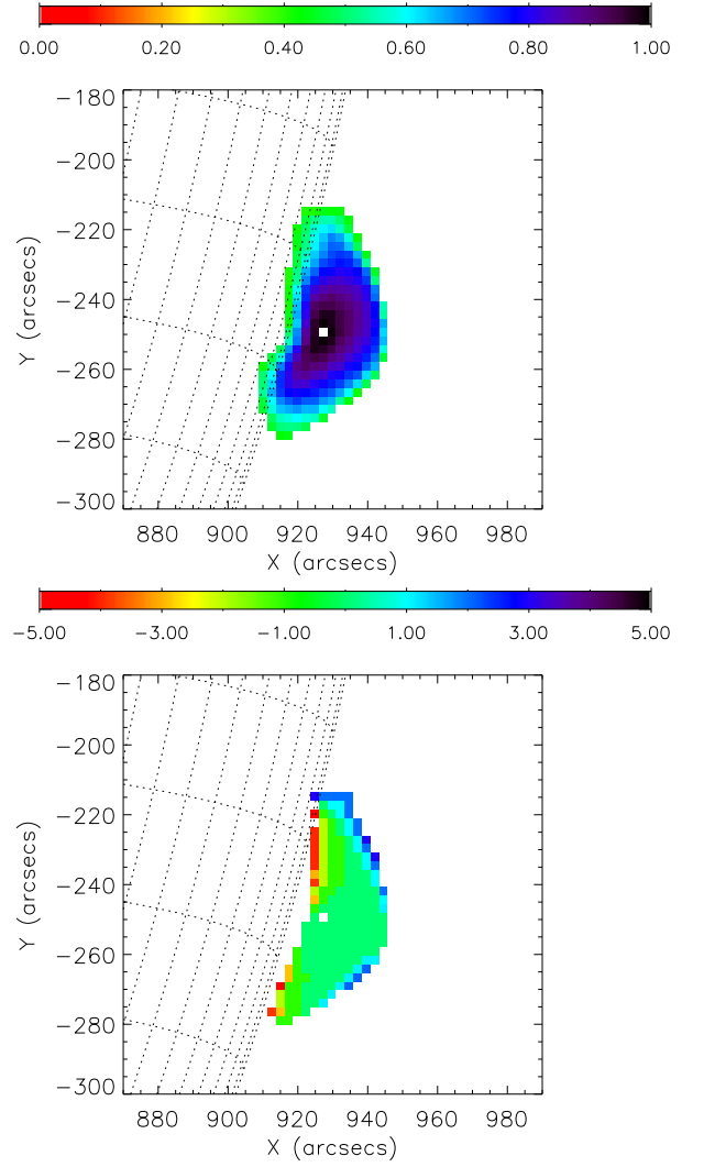
Fig. 8. Top: Cross-correlation coefficient map for background subtracted microwave emission at 17 GHz, obtained by the Nobeyama Radioheliograph during the pulsating regime of the limb flare of 8th May 1998. The correlation coefficient is calculated with zero time lag. The master pixel is the pixel with the highest time-integrated intensity of the signal. The bar shows the colour coding of the correlation coefficient. Bottom: Correlation time-lag map for microwave emission. The bar shows the colour coding of the time lag in seconds. In both panels the central white point corresponds to the master pixel.
