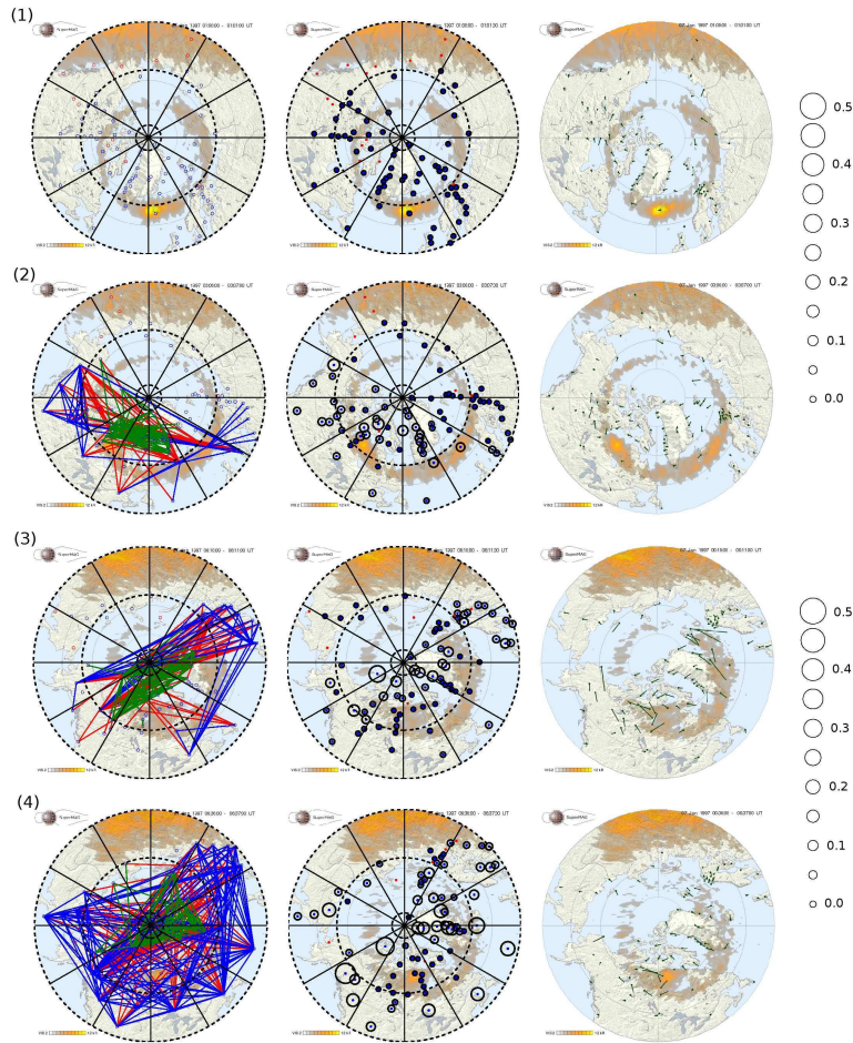
Figure S6. Connection maps, degree maps and VIS data in the same format as figure 4 (main text) for a 128 minute network at a 4 minute lag.
