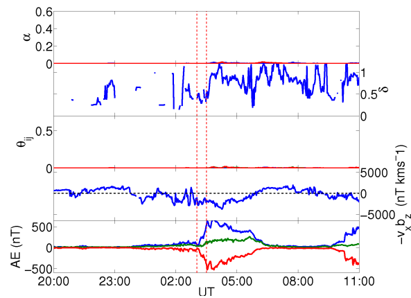
Figure S7. Network parameters describing the unique connections for the 4 minute lag network, \mathbf{A}_4^* , for substorm 1 03:03 7th January 1997. The figure has the same format and axis scaling as figure 3 (main text).
