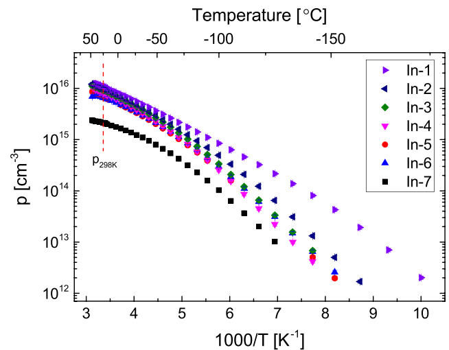
FIGURE 1 Carrier concentration versus temperature from Hall effect measurements. The values at 298 K were taken as the ionized indium concentrations for the lifetime measurements presented later [Colour figure can be viewed at wileyonlinelibrary.com ]
