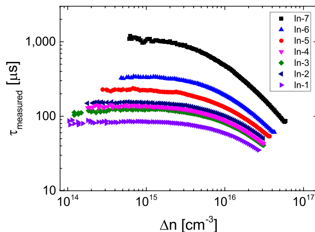
FIGURE 3 Measured lifetime versus excess carrier concentration in as-received indium doped silicon samples measured with superacid-derived surface passivation [Colour figure can be viewed at wileyonlinelibrary.com ]
