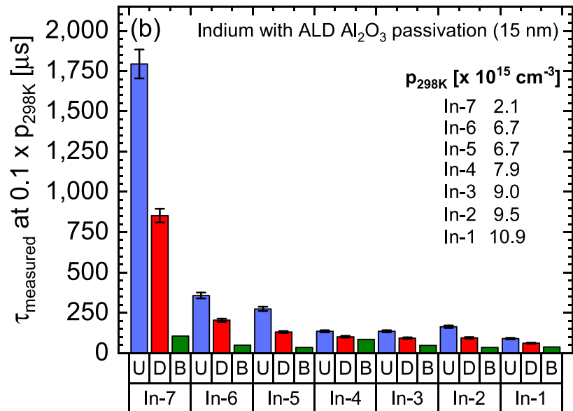
FIGURE 8 Measured effective lifetimes from LID experiments on ALD \text{Al}_2\text{O}_3 passivated indium doped samples. Graph (a) shows lifetime at an excess carrier density of 10^{15} \text{ cm}^{-3} versus time under \sim 1 Sun illumination for sample In-7, showing the original lifetime can be recovered by a 15 min anneal at 200^\circ\text{C} . The 2 \Omega\text{cm} n -type float-zone (FZ) control sample does not degrade under illumination. Graph (b) shows the undegraded (“U”) and degraded (“D”) lifetimes in all the indium doped silicon samples studied. Also shown in graph (b) are the degraded lifetimes for boron-doped samples (“B”) with the same doping level and oxygen concentration taken from the parameterization of Bothe et al. 44 Lifetimes in graph (b) are at an excess carrier density of 0.1 \times p_{298\text{K}} to facilitate direct comparison with Bothe et al’s data [Colour figure can be viewed at wileyonlinelibrary.com ]
