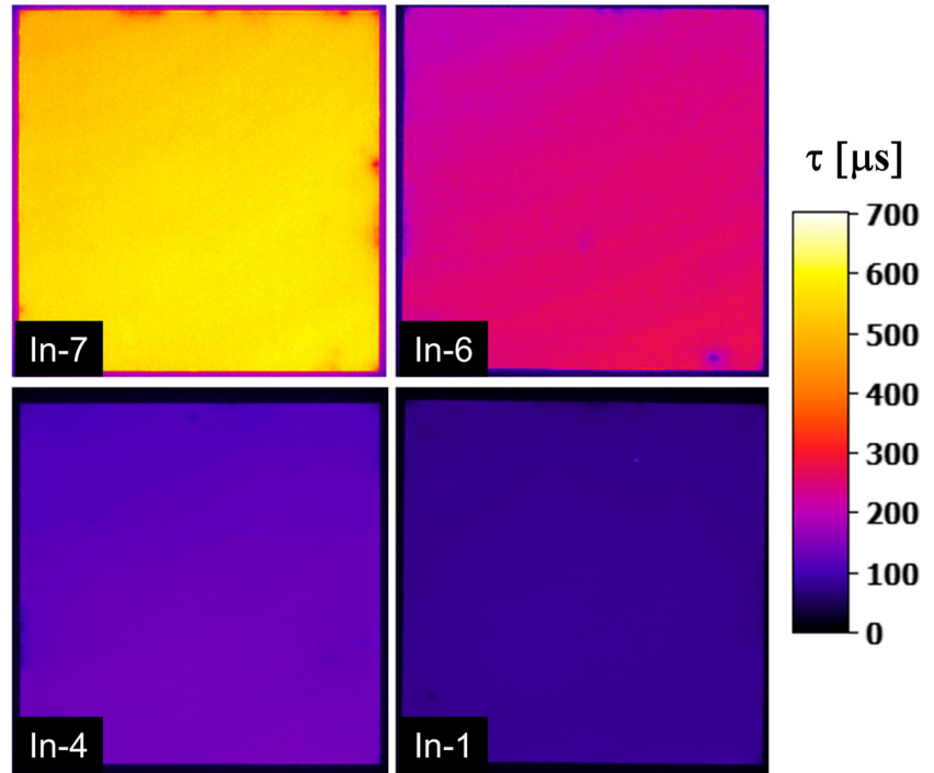
FIGURE 4 Calibrated PL lifetime images under 1 Sun illumination of selected as-received indium doped silicon samples (4 cm × 4 cm) measured with superacid-derived surface passivation. These images demonstrate the uniformity of both the surface passivation and the lifetime distribution in the sample [Colour figure can be viewed at wileyonlinelibrary.com ]
