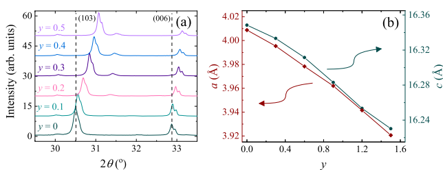
Figure 4. (a) Shift of the (103) and (006) diffraction peaks with increasing Co content y in \text{Fe}_{3-y}\text{Co}_y\text{GeTe}_2 . The splitting of the peaks is due to the presence of \text{Cu } K_{\alpha 1} and K_{\alpha 2} radiation in the X-ray source. (b) Variation of the lattice parameters a (left axis, red diamonds) and c (right axis, green circles) with the Co content y in \text{Fe}_{3-y}\text{Co}_y\text{GeTe}_2 .
