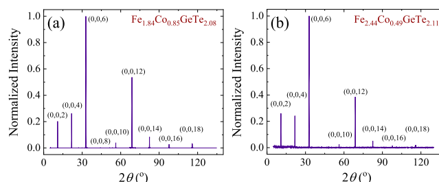
Figure 5. X-ray diffraction patterns obtained on single crystals with estimated compositions of (a) \text{Fe}_{1.84}\text{Co}_{0.85}\text{GeTe}_{2.08} and (b) \text{Fe}_{2.44}\text{Co}_{0.49}\text{GeTe}_{2.11} . The platelets were mounted with the ab plane parallel to the X-ray beam when the scattering angle was zero and the (00 l ) reflections observed are shown.
