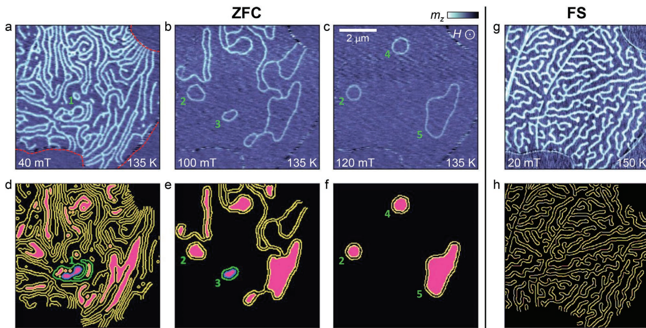
Figure 2. Seeding and emergence of isolated skyrmionium states from loop-like stripe domains. a–c) Scanning transmission X-ray micrographs of the \text{Fe}_{3-x}\text{GeTe}_2 x = 0.27 flake as a function of increasing applied magnetic field at 135 K, revealing the formation of skyrmionium states, labeled 1–5. The sample was initialized by zero-field cooling (ZFC) from above T_C . The color map is proportional to the out-of-plane magnetization component, m_z . d–f) Visualizations of the magnetic domain walls as determined by an edge detection algorithm. Regions representing loop-like states with the correct configuration to become isolated skyrmionium, or higher-order, states are highlighted by the magenta fill. One example skyrmionium emergence is shown by the highlighted green and blue domain walls in d and e. g, h) X-ray micrograph and domain wall view of the FGT flake following a field sweep (FS) procedure at 150 K, where the magnetic field was increased starting from a uniformly magnetized state at -250 mT. The lack of magenta-filled regions in the nucleated stripe domain state demonstrates a lack of potential composite skyrmion. The red dashed lines in a) indicate the edge of the flake sample.
