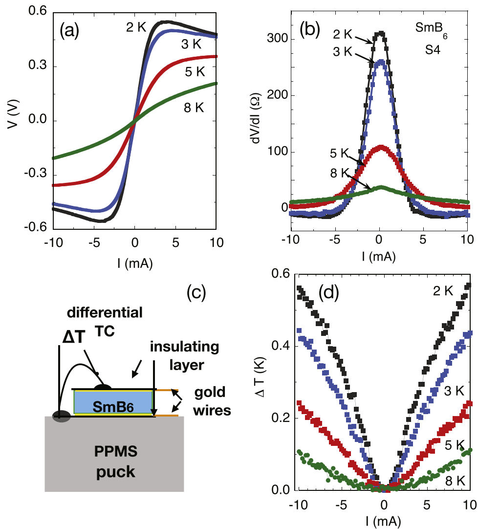
Fig. 6. (Color online)(a)- I - V curves for single crystal \text{SmB}_6 (sample S4) at various temperatures. (b)- dV/dI curves at the same temperatures. (c)- set-up used to measure \Delta T . (d)- self heating effect of dc current ( \Delta T vs. I ) measured for the same sample.
