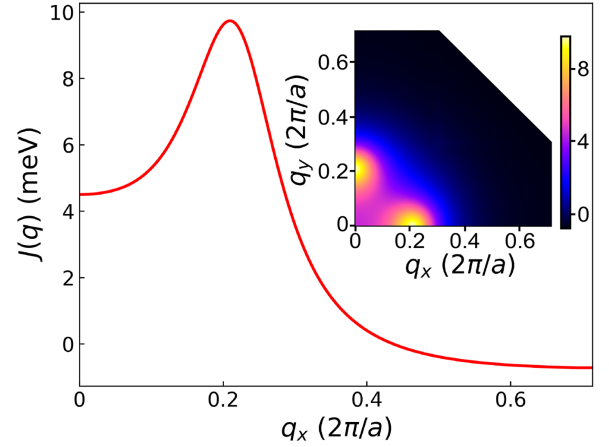
FIG. 5. Fourier transform J(q) of the magnetic interactions up to 60 unit cells. The inset shows a colormap of J(q) on the q_z = 0 plane of the Brillouin zone.
