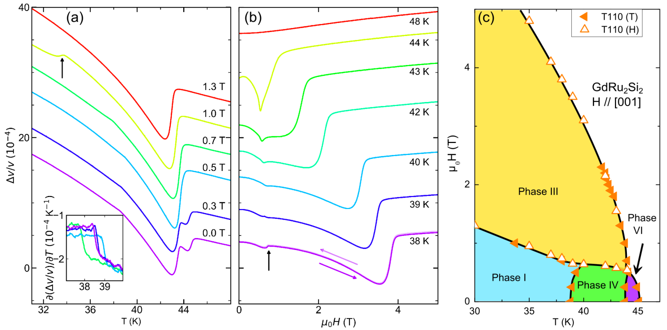
FIG. 2. Sound-velocity changes of the mode T110 vs temperature for selected magnetic fields (a), and vs field for selected temperatures (b). The curves are arbitrarily shifted along the y axis for clarity. (c) H - T phase diagram extracted from our ultrasound data, for magnetic fields applied along [001]. The black lines are guides to the eye.
