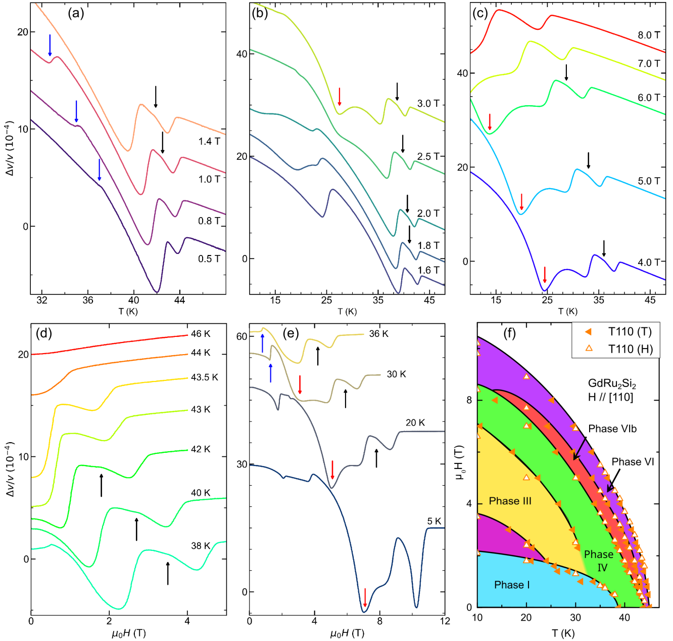
FIG. 3. Sound-velocity changes of the mode T110 vs temperature for selected magnetic fields (a)–(c), and vs field for selected temperatures (d) and (e). The curves are arbitrarily shifted along the y axis for clarity. (f) H - T phase diagram extracted from our ultrasound data, for magnetic fields applied along [110] . The black lines are guides to the eye.
