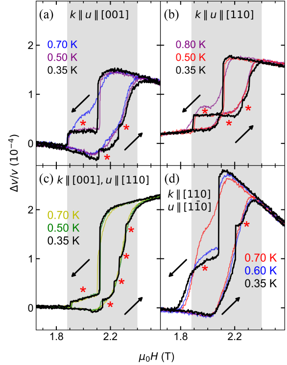
FIG. 1. Sound-velocity changes versus magnetic field at selected temperatures below 0.9 K, for the studied acoustic modes in GdRu 2 Si 2 : (a) \mathbf{k} \parallel \mathbf{u} \parallel [001] , (b) \mathbf{k} \parallel \mathbf{u} \parallel [110] , (c) \mathbf{k} \parallel [001] and \mathbf{u} \parallel [110] , and (d) \mathbf{k} \parallel [110] and \mathbf{u} \parallel [1\bar{1}0] . Magnetic field was applied along [001]. The skyrmion phase is indicated by the gray area, which we define as the region where up and down sweeps start to differ in (a). These phase boundaries are consistent with the results of Ref. [12] obtained at higher temperatures. The red stars show the different elasticity plateaus discussed in the text.
