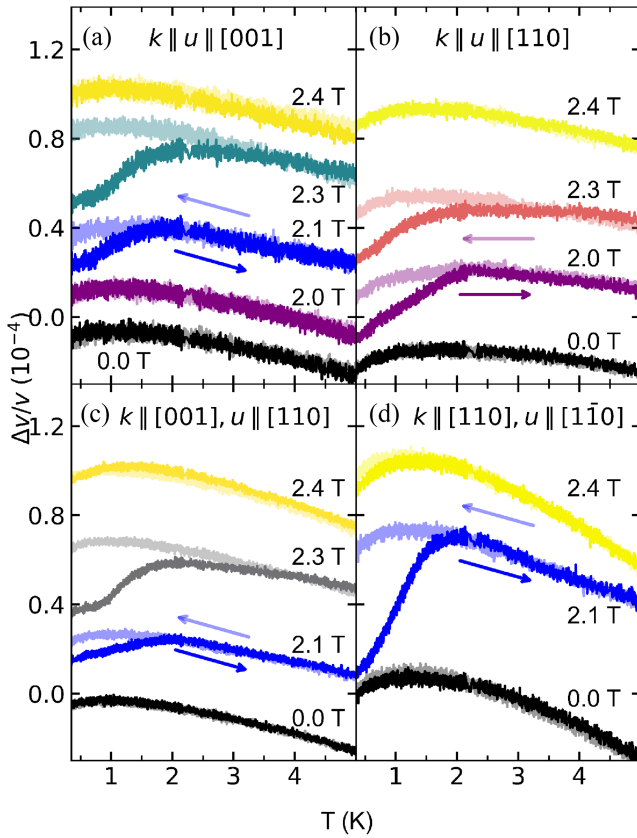
FIG. 4. Sound-velocity changes versus temperature at selected magnetic fields, for the studied elastic modes: (a) \mathbf{k} \parallel \mathbf{u} \parallel [001] , (b) \mathbf{k} \parallel \mathbf{u} \parallel [110] , (c) \mathbf{k} \parallel [001] and \mathbf{u} \parallel [110] , and (d) \mathbf{k} \parallel [110] and \mathbf{u} \parallel [1\bar{1}0] . The measurement were performed under zero-field-cooled (darker colored) and field cooled (lighter colored) conditions. The magnetic field was aligned along [001] . The curves are shifted along y-axis for clarity.
