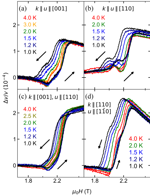
FIG. 2. Sound-velocity changes versus magnetic field at selected temperatures above 0.9 K, for the studied acoustic modes in \text{GdRu}_2\text{Si}_2 : (a) \mathbf{k} \parallel \mathbf{u} \parallel [001] , (b) \mathbf{k} \parallel \mathbf{u} \parallel [110] , (c) \mathbf{k} \parallel [001] and \mathbf{u} \parallel [110] , and (d) \mathbf{k} \parallel [110] and \mathbf{u} \parallel [1\bar{1}0] . Magnetic field was applied along [001] .
