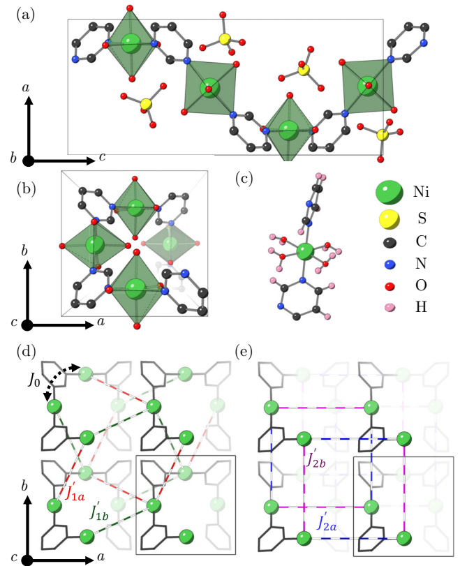
FIG. 1. The structure and exchange pathways of the S = 1 chiral chain in [\text{Ni}(\text{pym})(\text{H}_2\text{O})_4]\text{SO}_4 \cdot \text{H}_2\text{O} . (a) View looking down the b axis containing a single chiral chain connected by J_0 exchange mediating pym molecules (H atoms and \text{H}_2\text{O} molecules have been omitted for clarity). (b) View looking down the tetragonal P4_1 unit cell c axis depicting the fourfold rotation of the local Ni(II) octahedral environment. (c) The local crystal environment of each Ni(II) ion. (d) and (e) View down the c axis showing exchange pathways. The black dashed arrow represents the intrachain J_0 pathway. The red and green labeled dashed lines in (d) indicate the J'_{1a} and J'_{1b} interchain exchange interaction, respectively. In (e) the blue and purple labeled dashed lines denote the J'_{2a} and J'_{2b} interchain exchange interaction, respectively. The solid black lines indicate the unit cell boundaries.
