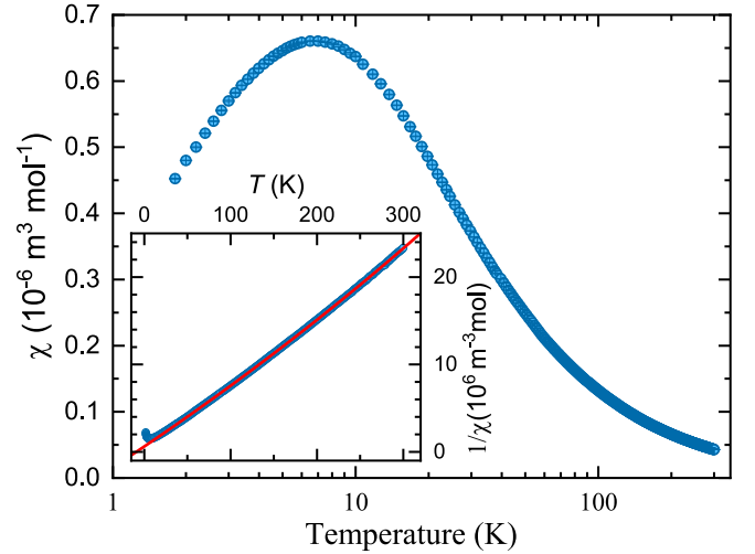
FIG. 2. Zero-field-cooled temperature-dependent magnetic susceptibility, \chi(T) , (blue circles) measured on powder samples of the S = 1 chiral chain, [\text{Ni}(\text{pym})(\text{H}_2\text{O})_4]\text{SO}_4 \cdot \text{D}_2\text{O} in an applied field of 0.1 T. Inset: The inverse susceptibility \chi^{-1} with a Curie-Weiss fit (red line).
