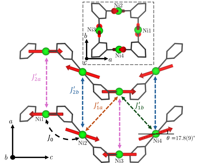
FIG. 7. Zero-field magnetic structure of the S = 1 chiral chain [\text{Ni}(\text{pym})(\text{D}_2\text{O})_4]\text{SO}_4 \cdot \text{D}_2\text{O} determined using elastic neutron diffraction and viewed looking down the b axis. The red arrows indicate the Ni(II) moments which are canted by \theta = 17.8(9)^\circ from the c axis and whose component in the ab plane rotates by 90^\circ from site to site along the chain yielding a chiral magnetic structure. Dashed lines indicate the magnetic exchange interactions. Inset: View of a single chain down the c axis showing chiral arrangement of the magnetic moments.
