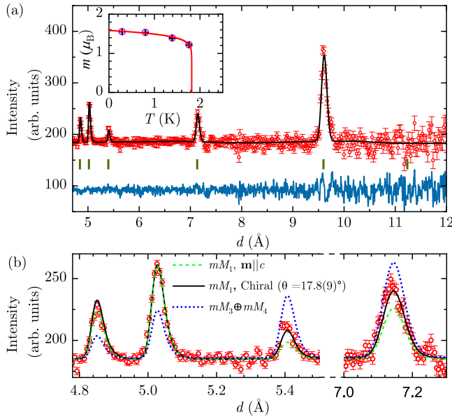
FIG. 5. (a) The magnetic powder diffraction pattern of [\text{Ni}(\text{pym})(\text{D}_2\text{O})_4]\text{SO}_4 \cdot \text{D}_2\text{O} , obtained by subtracting the nuclear structure contribution at 5.0(1) K from the 0.28(1) K data. The red circles represent the data, the black line shows the Rietveld fit of the chiral magnetic structure, the blue line is the difference and the green ticks mark the magnetic Bragg positions. Inset: T dependence of the ordered Ni(II) magnetic moment. (b) Comparison of the diffraction patterns produced by a collinear m||c , chiral and m||ab magnetic structures.
