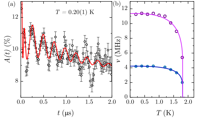
FIG. 4. (a) Representative \mu^+ SR spectra (black circles) measured at T = 0.20(1) K. (b) Temperature dependence of the muon spin precession frequencies (circles). Solid lines in both correspond to the fits to the data described in the text.
