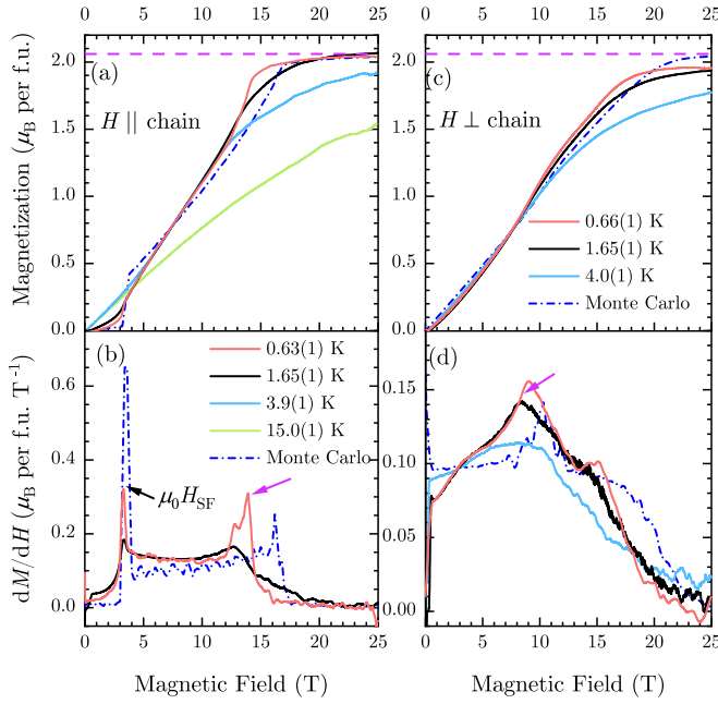
FIG. 3. Field-dependent magnetization, M(H) , of chiral S = 1 chain [\text{Ni}(\text{pym})(\text{H}_2\text{O})_4]\text{SO}_4 \cdot \text{H}_2\text{O} with the applied field (a) parallel and (c) perpendicular to the chain. Differential susceptibility, dM/dH , with applied field (b) parallel and (d) perpendicular to the chain. The purple dashed line shows the 0.63(1) K projected saturation value with H||c . The black arrow marks the spin-flop transition and the purple arrows indicate additional metamagnetic transitions. The blue dash-dot line in all panels shows the results of the classical Monte Carlo simulation described in Sec. III F.
