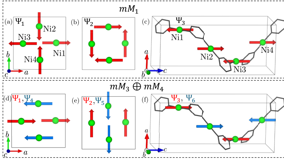
FIG. 6. Magnetic basis vectors \Psi_i transformed by the symmetries of the mM_1 irreducible representation (a)–(c) and the mM_3 \oplus mM_4 irreducible representation (d)–(f), shown for the four Ni(II) sites in the P4_1 unit cell of [\text{Ni}(\text{pym})(\text{D}_2\text{O})_4]\text{SO}_4 \cdot \text{D}_2\text{O} . Red and blue arrows indicate the magnetic moments and solid black lines show the crystallographic unit cell boundaries.
