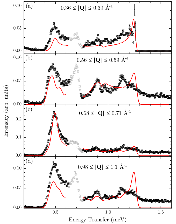
FIG. 9. Representative line cuts of the inelastic neutron scattering data for [\text{Ni}(\text{pym-D}_4)(\text{D}_2\text{O})_4]\text{SO}_4 \cdot \text{D}_2\text{O} . The data are integrated over (a) 0.36 \leq |\mathbf{Q}| \leq 0.39 \text{ \AA}^{-1} , (b) 0.56 \leq |\mathbf{Q}| \leq 0.59 \text{ \AA}^{-1} , (c) 0.68 \leq |\mathbf{Q}| \leq 0.71 \text{ \AA}^{-1} , and (d) 0.98 \leq |\mathbf{Q}| \leq 1.1 \text{ \AA}^{-1} . The red lines are modeled using Eq. (1) and the parameters J_0 = 6.81(1) K, J'_{1a} = -0.09(1) K, and D = -3.02(1) K, determined by fitting the full 2D dataset. Data points are shown as black circles, and the gray circles indicate the data masked during fitting.
