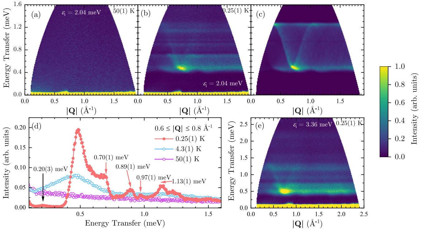
FIG. 8. Time of flight powder inelastic neutron scattering (INS) spectra of [\text{Ni}(\text{pym-D}_4)(\text{H}_2\text{O})_4]\text{SO}_4 \cdot \text{H}_2\text{O} taken at (a) 50(1) K and (b) 0.25(1) K with \epsilon_i = 2.04 meV. (c) Powder averaged linear spin wave theory simulations of the spin-wave spectra using the Hamiltonian in Eq. (1) and the parameters J_0 = 6.81(1) K, J'_{1a} = -0.09(1) K, and D = -3.02(1) K. (d) Line cut of the spectra observed at various temperatures, integrated over 0.6 < |\mathbf{Q}| < 0.8 \text{ \AA}^{-1} . (e) Inelastic neutron scattering spectra collected at 0.25(1) K with \epsilon_i = 3.36 meV.
