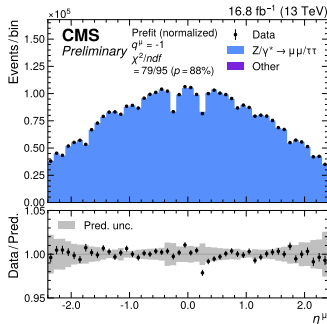
(b) \mu^- (pfit normalized)
