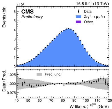
(a) prefit (normalized)
