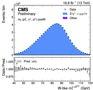
(b) postfit ( p_T^{\mu}, \eta^{\mu}, q^{\mu} )
