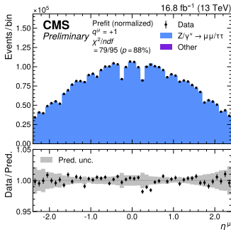
(a) \mu^+ (pfit normalized)
