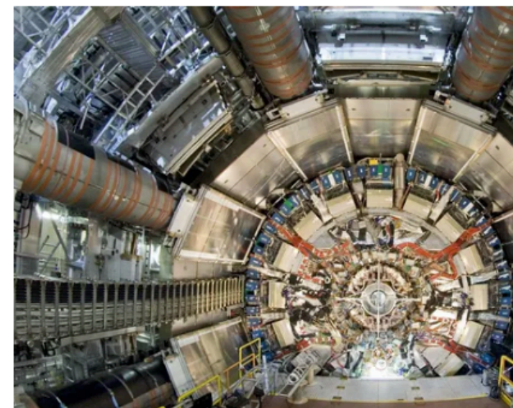
The ATLAS instrument at CERN's Large Hadron Collider has detected millions of Higgs boson particles. (Image credit: CERN/Claudia Marcelloni/Max Brice)
