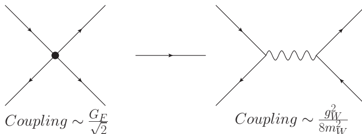
Figure 3: Weak coupling factor from weak interaction in the Fermi contact interaction picture, and the W-boson exchange picture.
