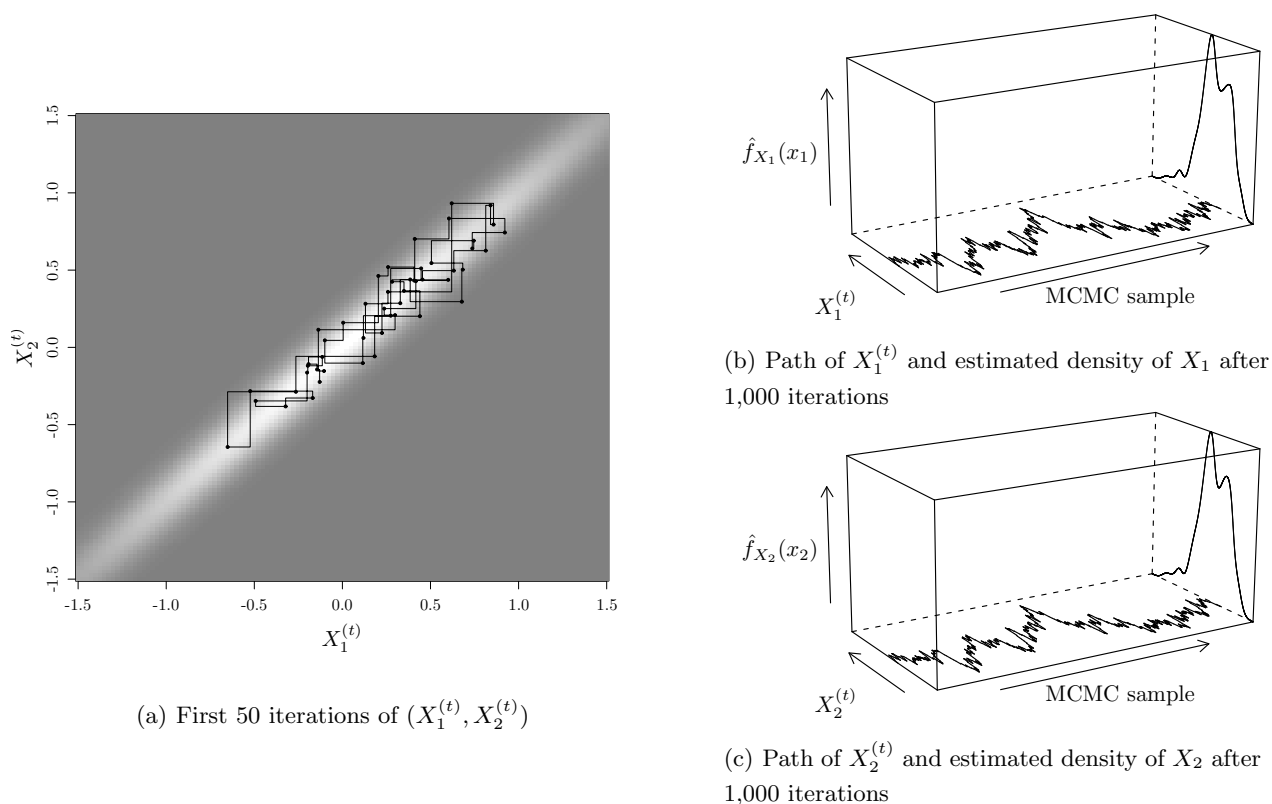
Fig. 3.5. Gibbs sampler for a bivariate normal distribution with correlation \rho(X_1, X_2) = 0.99
