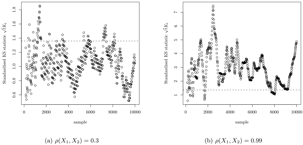
Fig. 3.13. Standardised Kolmogorov-Smirnov statistic for X_1^{(5 \cdot t)} from the Gibbs sampler from the bivariate Gaussian for two different correlations.
