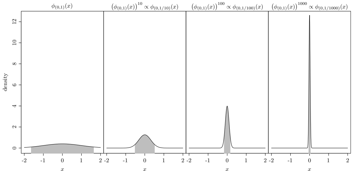
Fig. 3.16. Density of the \mathbf{N}(0, 1) raised to increasing powers. The areas shaded in grey represent 90% of the probability mass.
