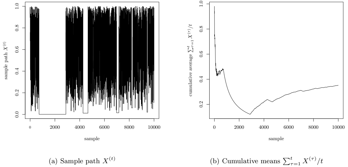
Fig. 3.12. Sample paths and cumulative means obtained for the pathological Beta generator, \alpha = 1 .
