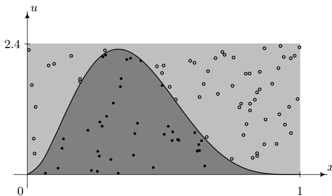
Fig. 2.2. Illustration of Example 2.3. Sampling from the area under the curve (dark grey) corresponds to sampling from the Beta (3, 5) density. In Example 2.3 we use a uniform distribution over the light grey rectangle as a proposal distribution. Empty circles denote rejected values, filled circles denote accepted values.
