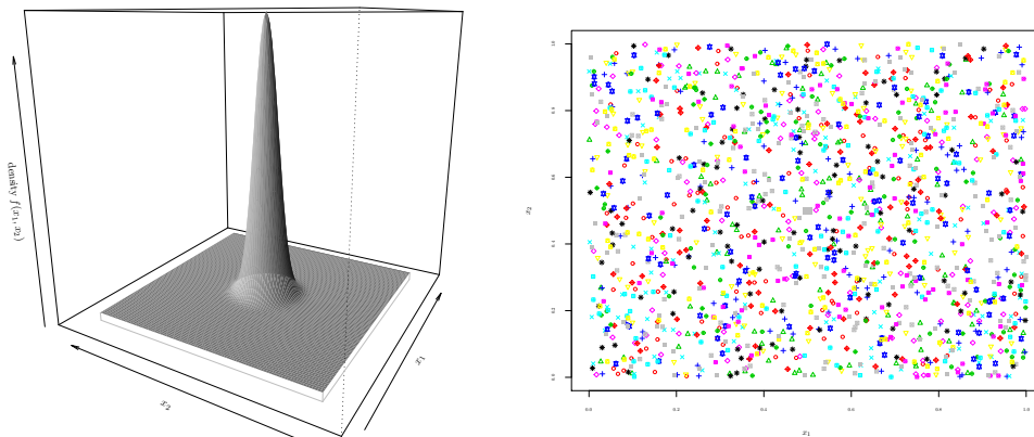
(a) Density for \delta = 0.2 , \boldsymbol{\mu} = (0.5, 0.5)' , and \sigma = 0.05 (b) First 100 values from 15 samples using different starting values. ( \delta = 10^{-3} , \boldsymbol{\mu} = (0.5, 0.5)' , and \sigma = 10^{-5} )
