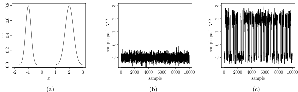
Fig. 3.11. Density of the mixture distribution with two random walk Metropolis samples using two different variances \text{Var}[\varepsilon] of the proposal. (a) Density f(x) . (b) Sample path of a random walk Metropolis algorithm with proposal variance \text{Var}[\varepsilon] = 0.4^2 . (c) Sample path of a random walk Metropolis algorithm with proposal variance \text{Var}[\varepsilon] = 1.2^2 .
