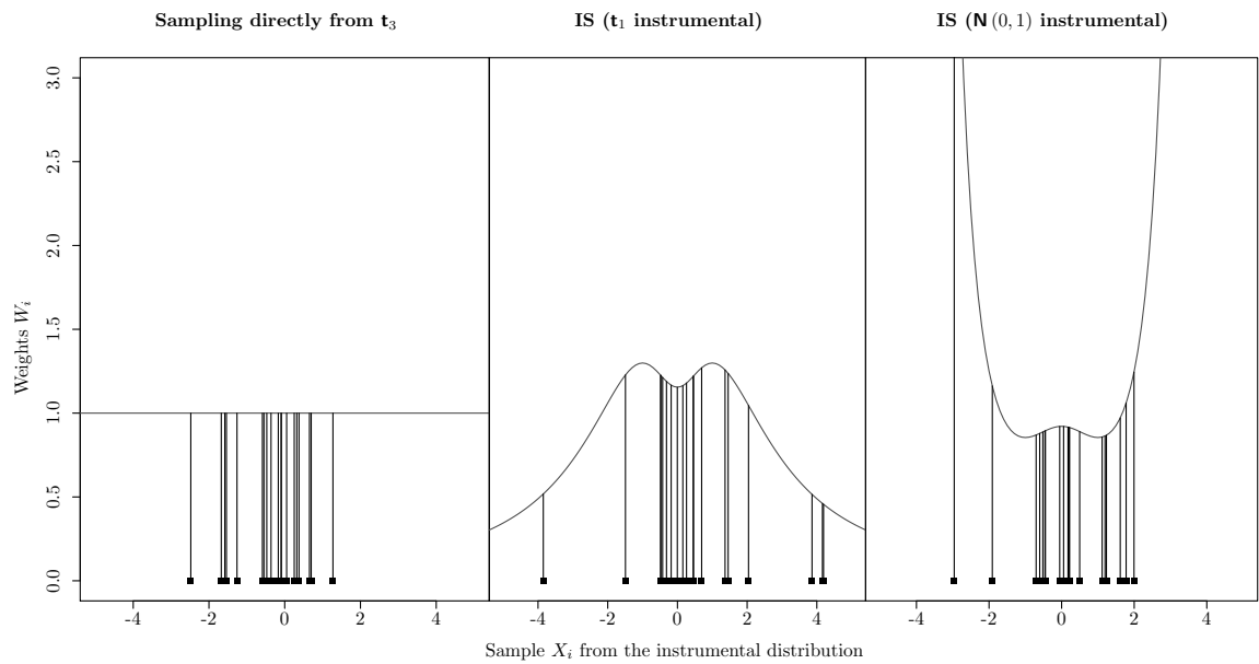
Fig. 2.6. Weights W_i obtained for 20 realisations X_i from the different proposal distributions.
