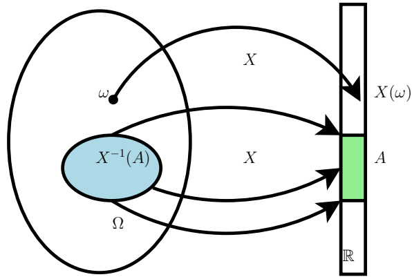
Fig. B.1. Random variables as functions from the sample space, \Omega , to \mathbb{R} . If \omega occurs in an experiment then X will be measured as having the value X(\omega) . If we want to know whether X takes a value in the set A (the green rectangle) then we need to check whether \omega takes a value which X maps into A , this set is often denoted X^{-1}(A) and corresponds to the blue ellipse here.
