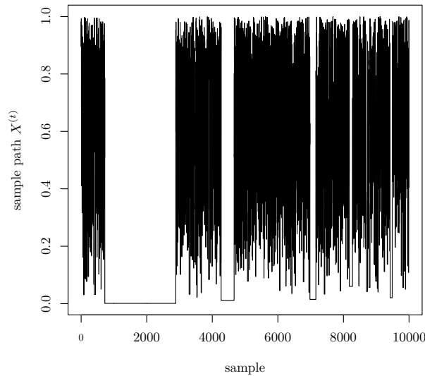
Figure 3.24: Sample path X^{(t)} obtained for the pathological Beta generator, \alpha = 1 .
