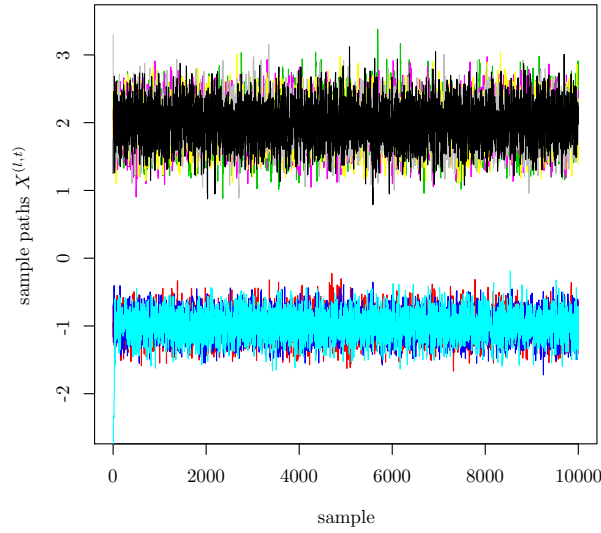
Figure 3.29: Comparison of the sample paths for L = 8 chains for the mixture of two Gaussians: \text{Var}[\varepsilon] = 1.2^2 .
