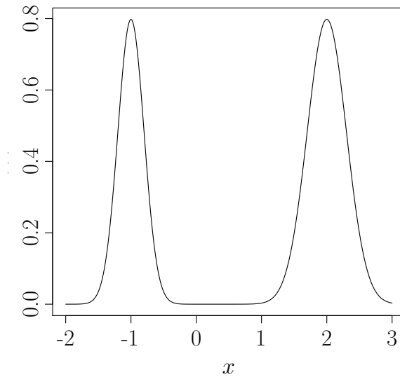
Figure 3.21: Density of a mixture distribution f(x) .
