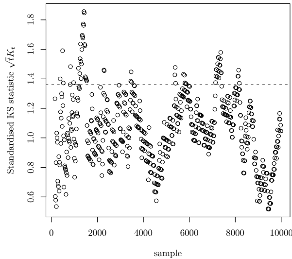
Figure 3.26: Standardised Kolmogorov–Smirnov statistic for X_1^{(5 \cdot t)} from the Gibbs sampler from the bivariate Gaussian, \rho(X_1, X_2) = 0.3 .
