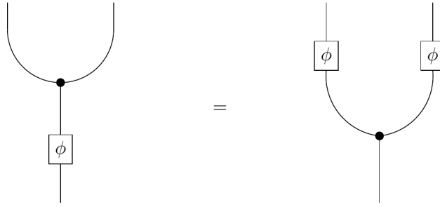
Figure B.12: Determinism.
