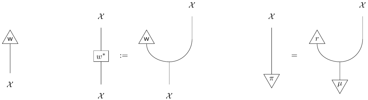
Figure B.14: Effects and reweighing.
