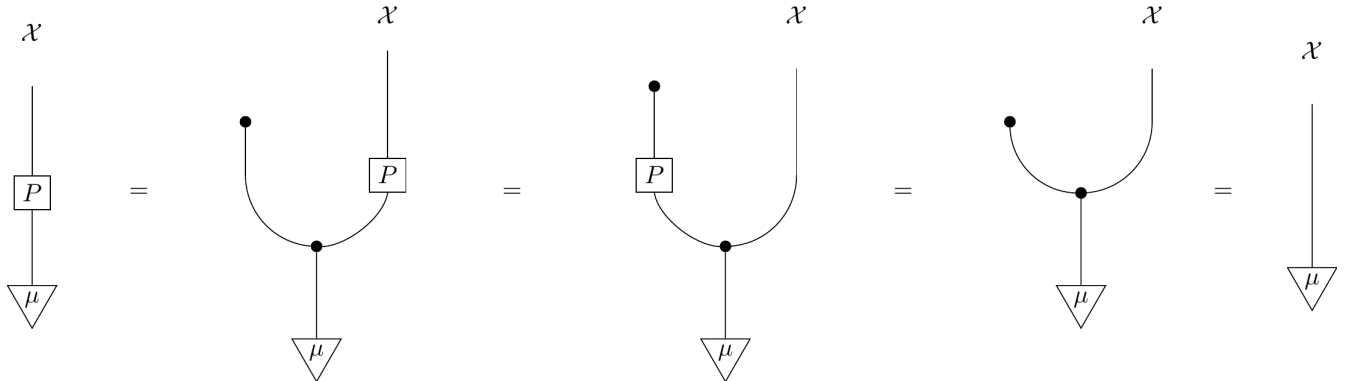
Figure B.10: Proof of proposition.
