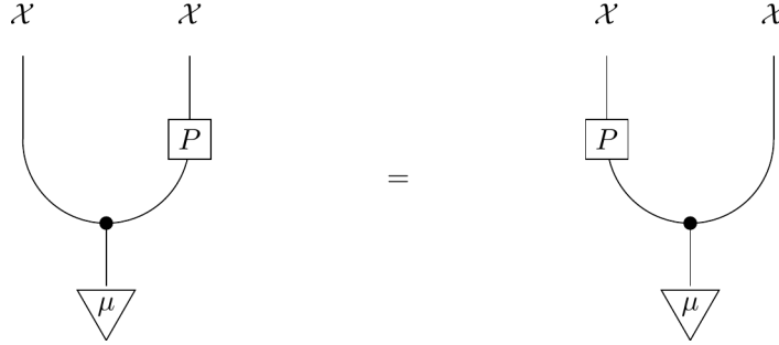
Figure B.9: Reversibility.
