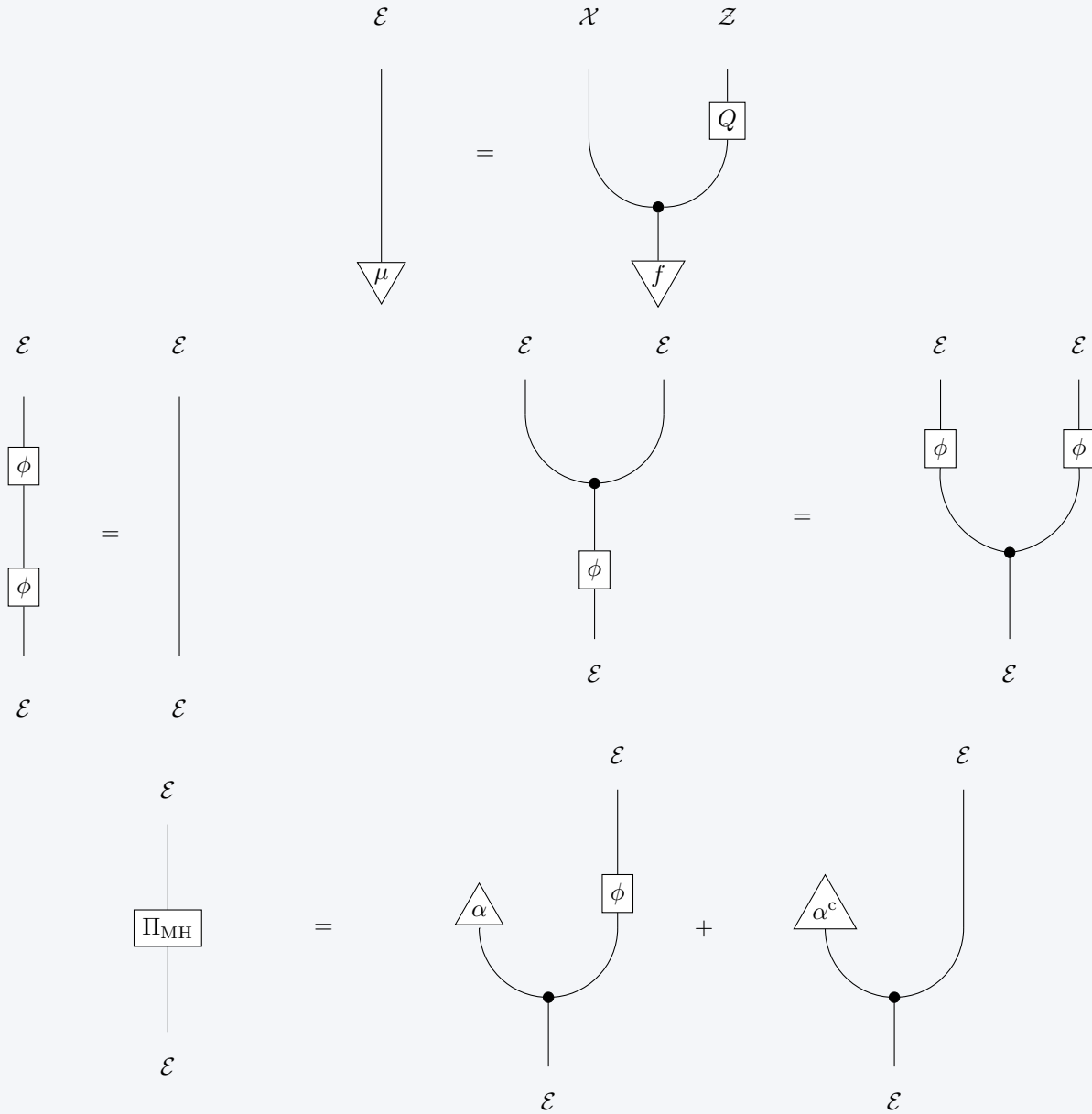
Figure 3.16: Abstract MH kernel on the augmented space
