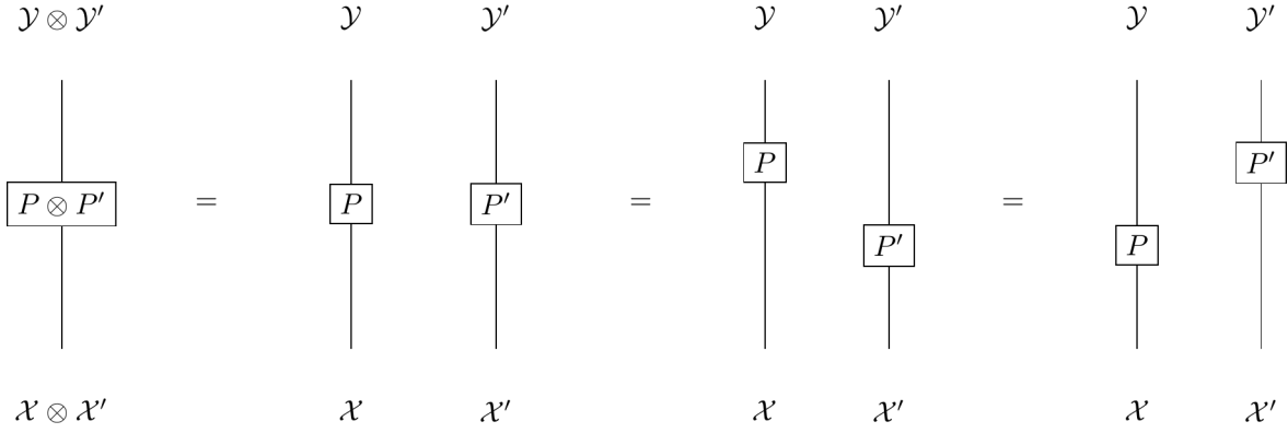
Figure B.2: Parallel composition.
