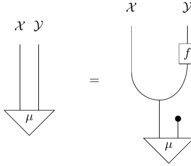
Figure B.11: A conditional.
