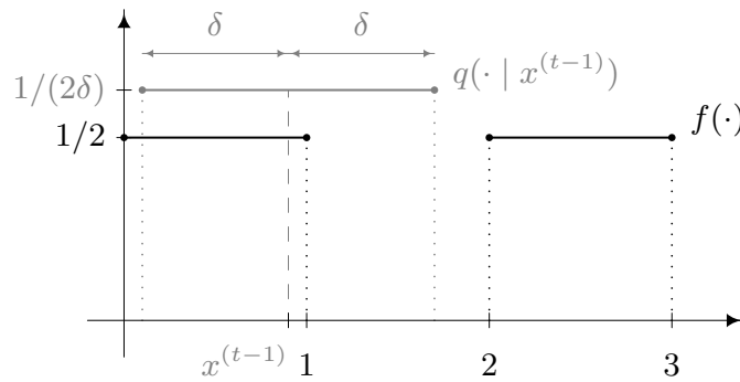
Figure 3.11: Illustration of Reducible Metropolis-Hastings.
