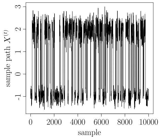
Figure 3.23: Sample path of a random walk Metropolis algorithm with proposal variance 1.2^2 and mixture distribution target.
