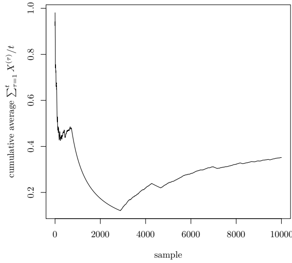
Figure 3.25: Cumulative mean \sum_{\tau=1}^t X^{(\tau)}/t obtained for the pathological Beta generator, \alpha = 1 .
