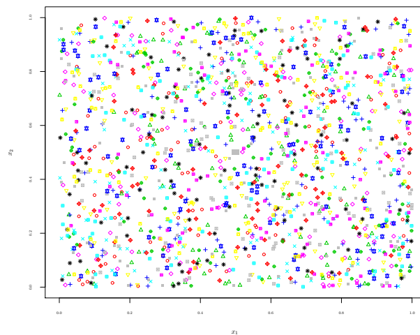
Figure 3.31: Witch's hat distribution: First 100 values from 15 samples using different starting values. \delta = 10^{-3} , \boldsymbol{\mu} = (0.5, 0.5)' , and \sigma = 10^{-5} .
