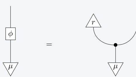
Figure 3.19: Radon–Nikodym condition.
