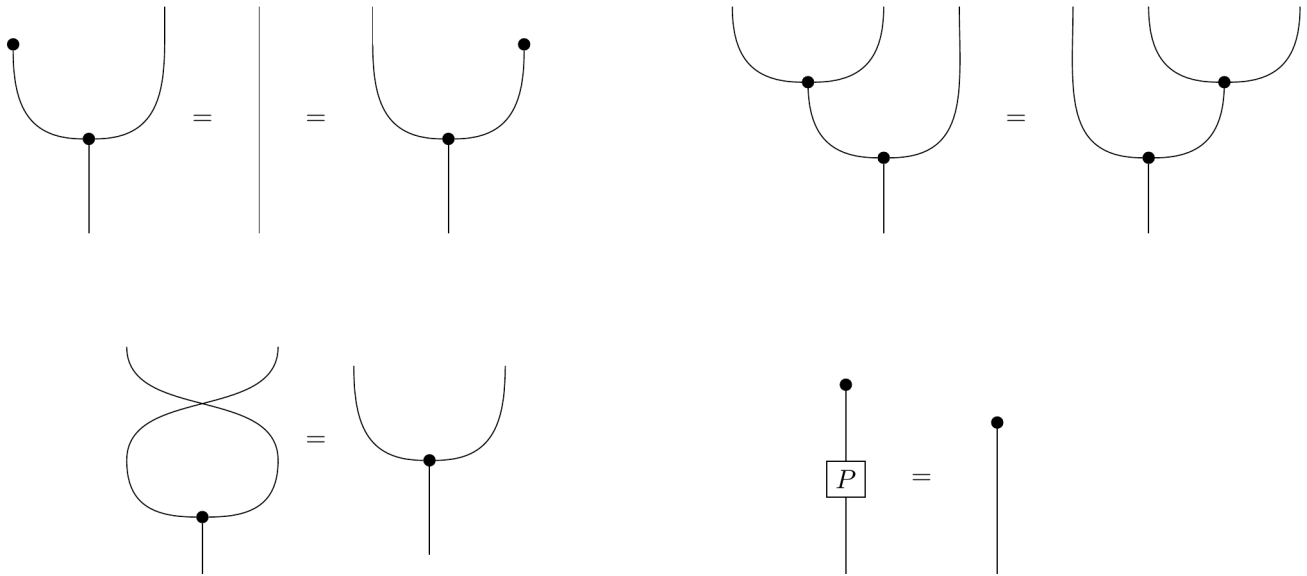
Figure B.5: Delete and swap properties.
