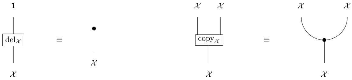
Figure B.4: Delete and copy.
