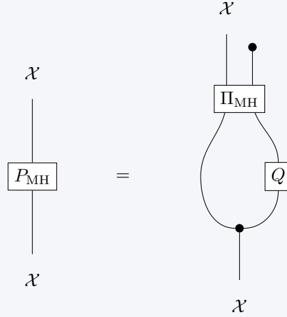
Figure 3.17: Abstract MH kernel on the original space
