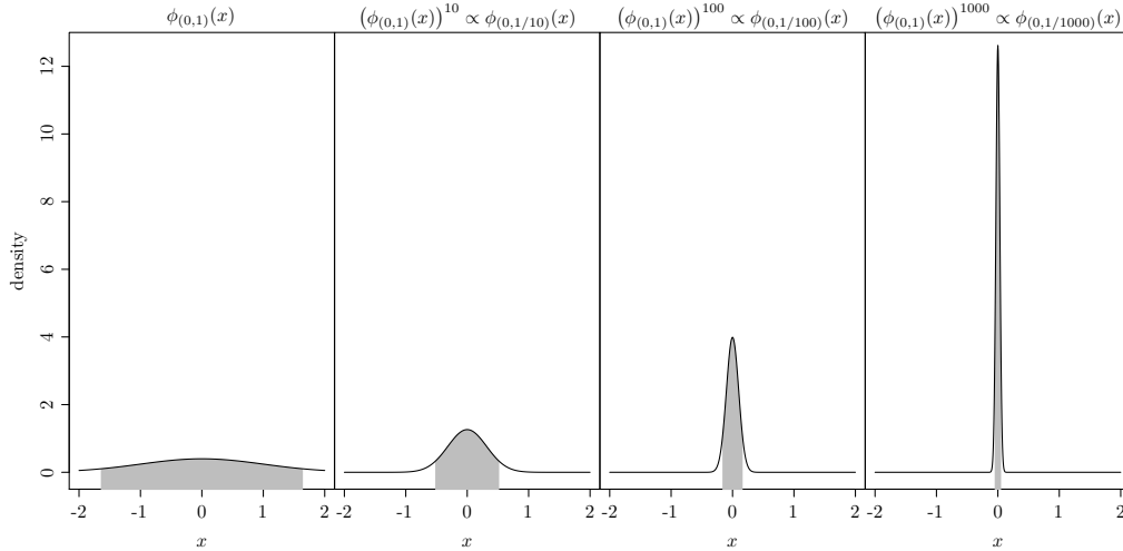
Figure 3.32: Density of the N(0,1) raised to increasing powers. The areas shaded in grey represent 90% of the probability mass.
