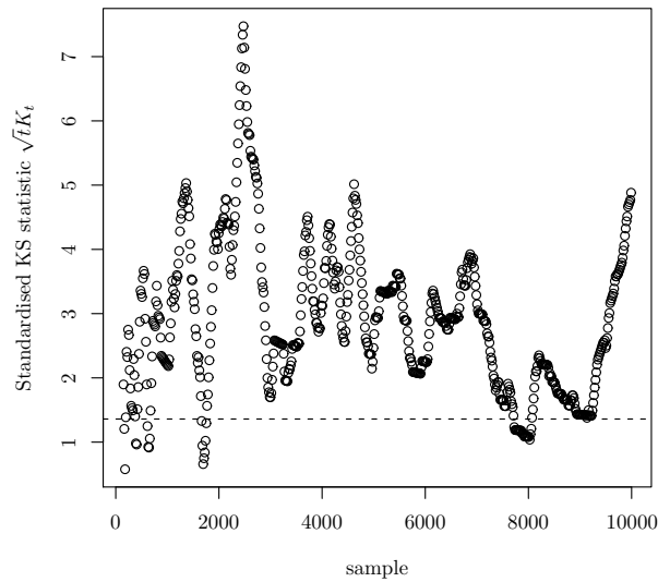
Figure 3.27: Standardised Kolmogorov–Smirnov statistic for X_1^{(5 \cdot t)} from the Gibbs sampler from the bivariate Gaussian, \rho(X_1, X_2) = 0.99 .
