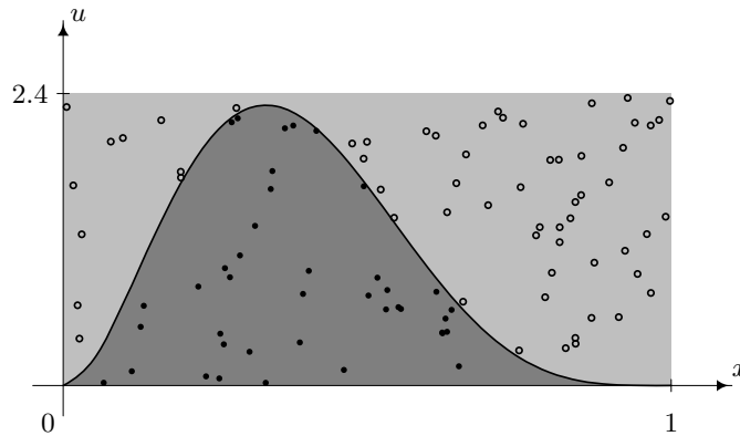
Figure 2.2: Sampling from the area under the curve (dark grey) corresponds to sampling from the Beta (3, 5) density. We use a uniform distribution over the light grey rectangle as a proposal distribution. Empty circles denote rejected values, filled circles denote accepted values.
