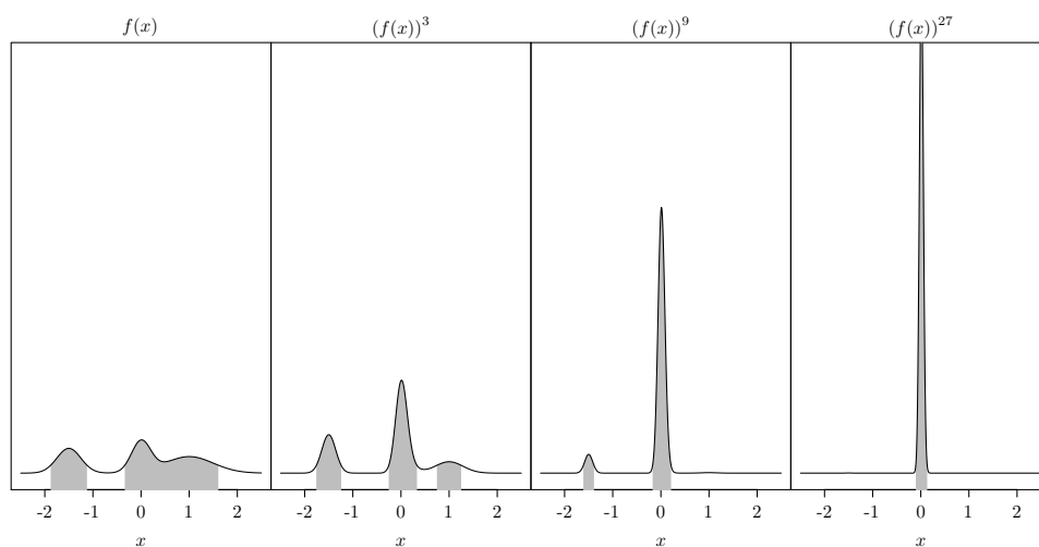
Figure 3.33: An arbitrary multimodal density raised to increasing powers. The areas shaded in grey reach from the 5% to the 95% quantiles.
