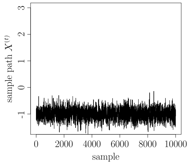
Figure 3.22: Sample path of a random walk Metropolis algorithm with proposal variance 0.4^2 and mixture distribution target f(x) .
