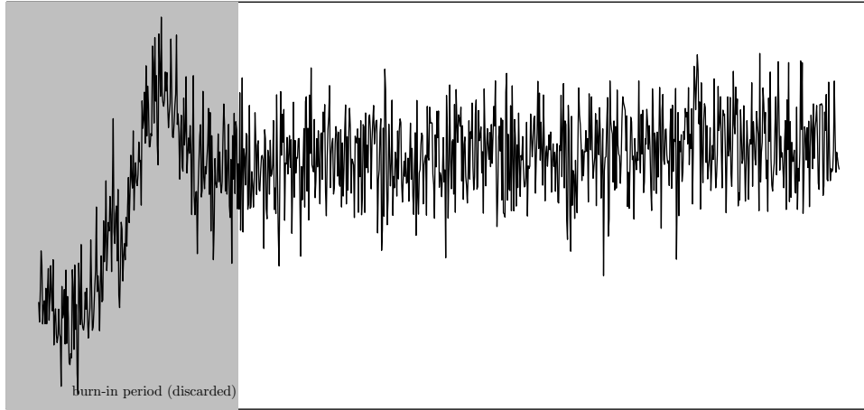
Figure 3.20: Illustration of the idea of a burn-in period.
