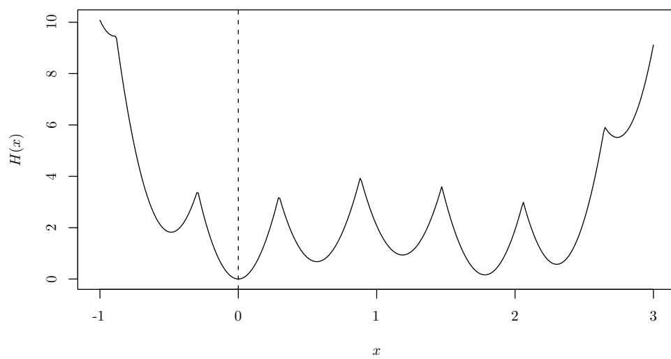
Figure 3.36: Objective function H(x) .
