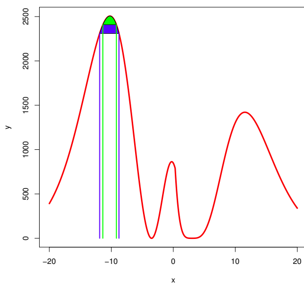
Figure 3.34: Simulated annealing for a continuous density.
