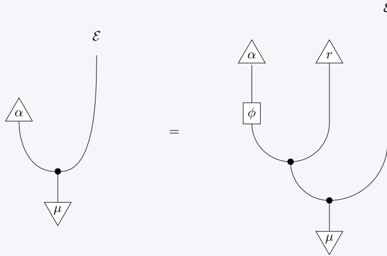
Figure 3.18: Necessary and sufficient condition for reversibility.
