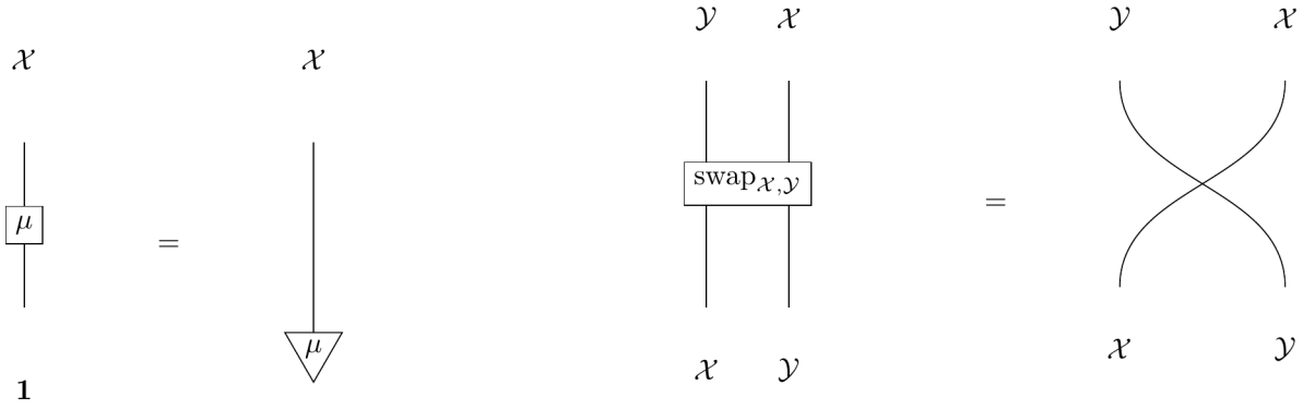
Figure B.3: States and swap.
