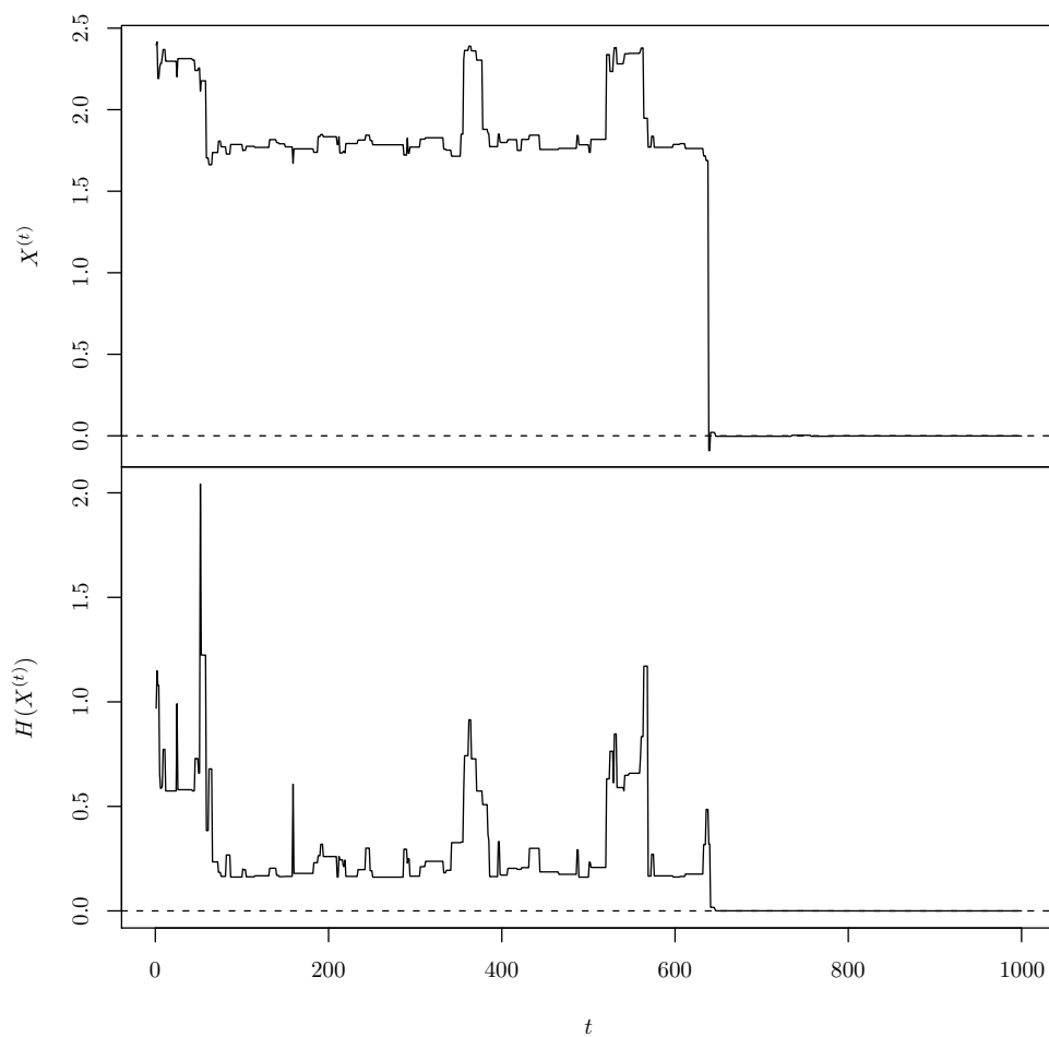
Figure 3.37: First 1,000 iterations of the Markov chain yielded by simulated annealing for finding the maximum of H(x) .
