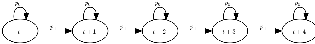
Figure A.4: A random walk on the positive integers.
