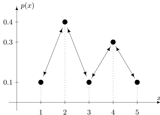
Figure 3.35: Illustration of a random walk Metropolis algorithm for the optimisation problem.
