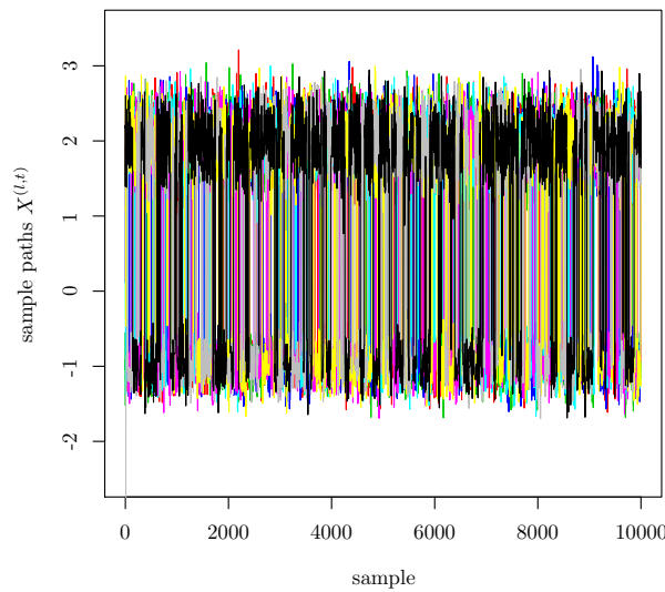
Figure 3.28: Comparison of the sample paths for L = 8 chains for the mixture of two Gaussians: \text{Var}[\varepsilon] = 0.4^2 .
