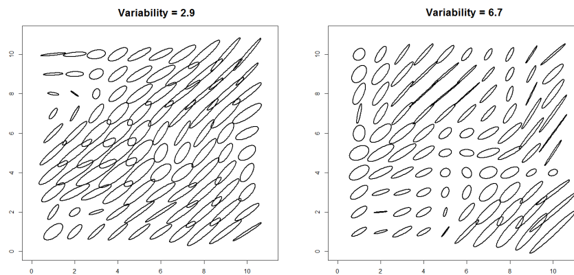
(b) Field realization with \zeta = 2.9
