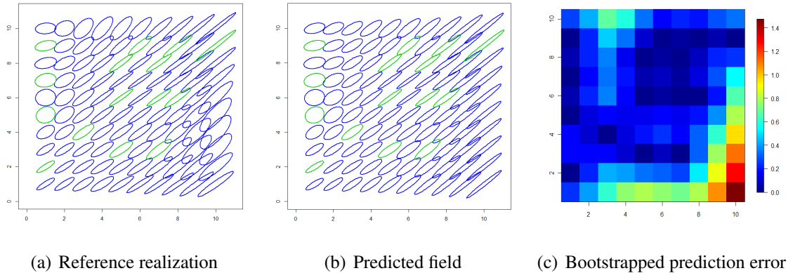
Figure 1: Panels (a) and (b): Comparison between the reference realization of the matrix field and the predicted field. Each positive definite matrix is represented by an ellipse centered in the respective location. Observed data are represented in green. Panel (c): Estimated expected prediction error.
