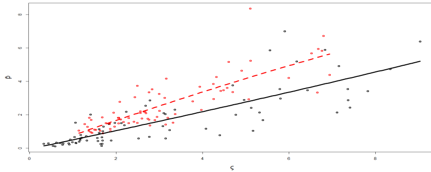
(a) Prediction error and variability
