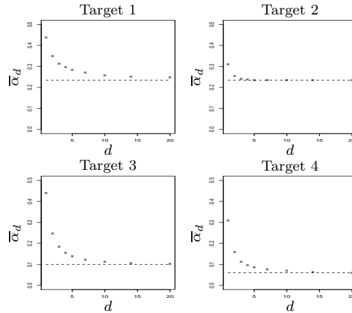
Figure 2: Plots of the optimal EAR \hat{\alpha} against dimension for Example Targets 1-4 using a Gaussian jump proposal. The horizontal dotted line approximates the apparent asymptotically optimal acceptance rate of 0.234 in the first two plots and 0.10 and 0.06 in the third and fourth plots respectively.
