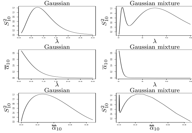
Figure 1: Plots for a Gaussian target (left) and the Gaussian mixture target of (11) with p_d = 1/d^2 (right), both at d = 10 and with a Gaussian jump proposal. Panels from top to bottom are (i) ESJD against scaling, (ii) EAR against scaling, and (iii) ESJD against EAR.
