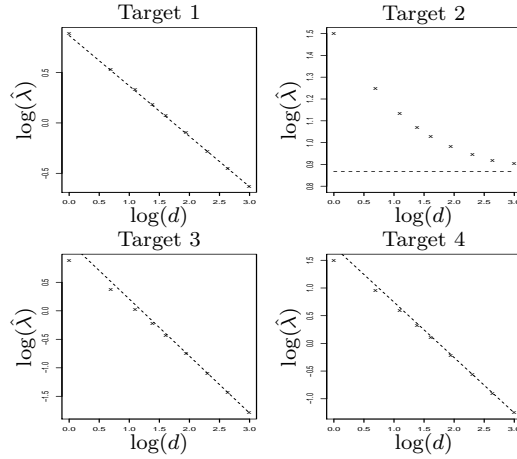
Figure 4: Plots of \log \hat{\lambda} against \log d for Target Examples 1-4. Optimal values predicted using Corollary 4 appear as dotted lines.
