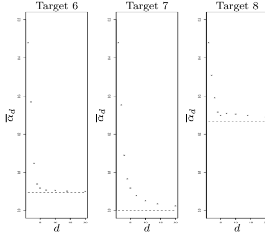
Figure 3: Plots of the optimal EAR \hat{\alpha}_d against dimension for Example Targets 6-8 using a Gaussian jump proposal. The horizontal dotted line in each plot represents the apparent asymptotically optimal acceptance rate of 0.234/5, 0, and 0.234 respectively.
