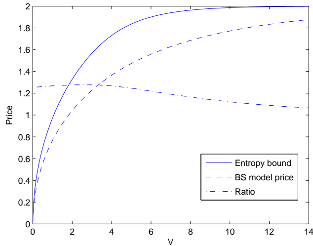
Figure 6: A plot of E(V) (the Black-Scholes model-based price, dashed line) and \tilde{J}(V/2) the entropy-based bound (solid line), scaled such that p = 1 . The ratio between these prices is also shown; for small V the limit ratio is \sqrt{\pi/2} , for large V the limit is 1. We have 0 \leq E(V) \leq H(\mu, \nu) \leq \tilde{J}(V/2) \leq 2 \wedge \sqrt{2V} . It should be noted that most plausible parameter combinations are represented by low values of V , so the left-hand side of this figure is the most relevant.
