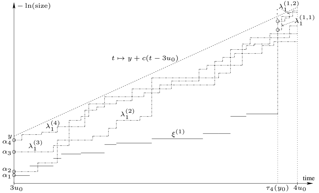
Figure 5-5: Illustration of the induction argument based on (5.33) for n = 3 and with y := c3u_0 in the case of a finite dislocation measure. By induction hypothesis N_{3u_0}^0 \geq 4 . The fragmentation property implies that the blocks alive at time 3u_0 start independent copies of \Pi^x (with different initial configurations). In this illustration we depict a realisation of these independent copies. For k \in \{1, \dots, 4\} set \alpha_k := -\ln(\lambda_k^0(3u_0)) . Then \xi^{(1)} is an independent copy of the subordinator \xi , shifted by \alpha_1 , and \lambda_1^{(k)} , k \in \{2, 3, 4\} , is an independent copy of (\lambda_1^{\alpha_k}(t))_{t \in [0, u_0]} . Further, the random variable \tau_4(y_0) - 3u_0 is an independent copy of \tau(y_0) . In view of the extended fragmentation property, \lambda_1^{(1,1)} and \lambda_1^{(1,2)} are independent copies of \lambda_1 , starting at \tau_4(y_0) and shifted by \xi^{(1)}(\tau_4(y_0))\Delta_1(\tau_4(y_0)) and \xi^{(1)}(\tau_4(y_0))\Delta_2(\tau_4(y_0)) respectively.
