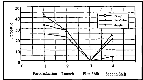
Fig. 12. Root cause patterns for the dimensional faults caused by design, installation and suppliers.
