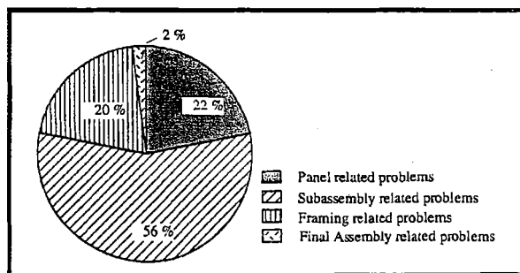
Fig. 14. Root cause classification based on the localization of the dimensional faults within the assembly process.
