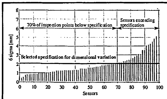
Fig. 3. Example of percentile chart for dimensional variation evaluation.
