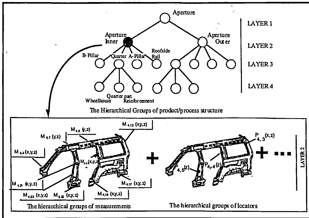
Fig. 5. The knowledge representation of the automotive body assembly.
