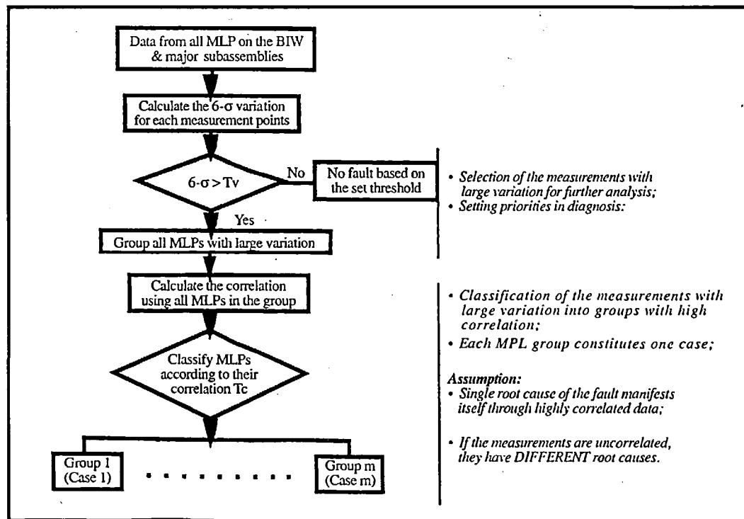
Fig. 6. The flow chart of diagnostic reasoning: fault detection.
