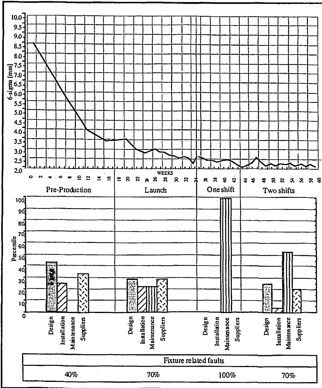
Fig. 4. Root causes classification based on the four production phases.
