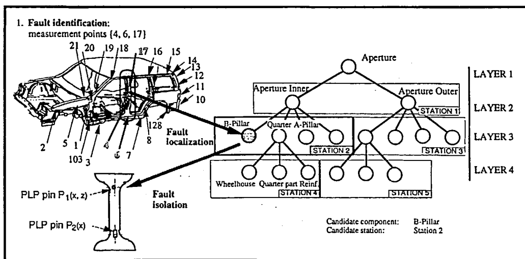
Fig. 7. The fault identification, localization, and isolation procedure.
