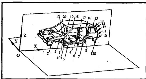
Fig. 1. The body coordinate system with an example of sensor locations.
