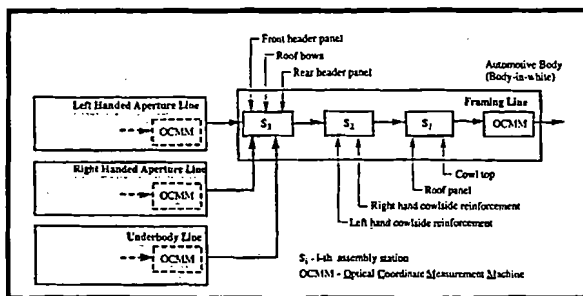
Fig. 2. Outline of the assembly process: critical stations of the framing line.
