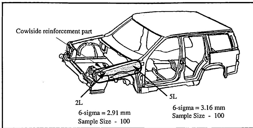
Fig. 8. Body-in-white with marked Cowlside panel and measurement sensors 2L & 5L.
