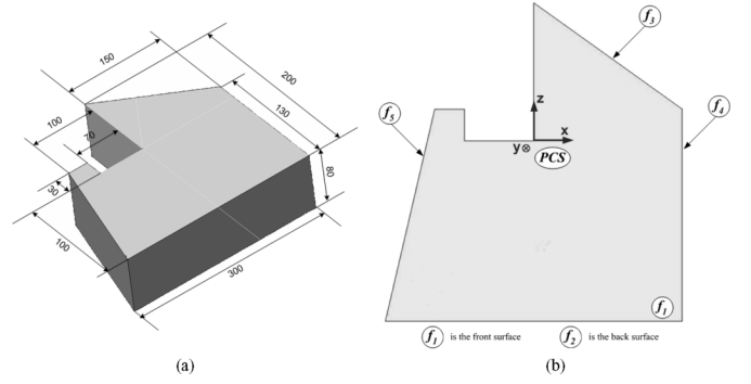
Fig. 9. Workpiece for the case study. (a) Isometric view. (b) Top view.
