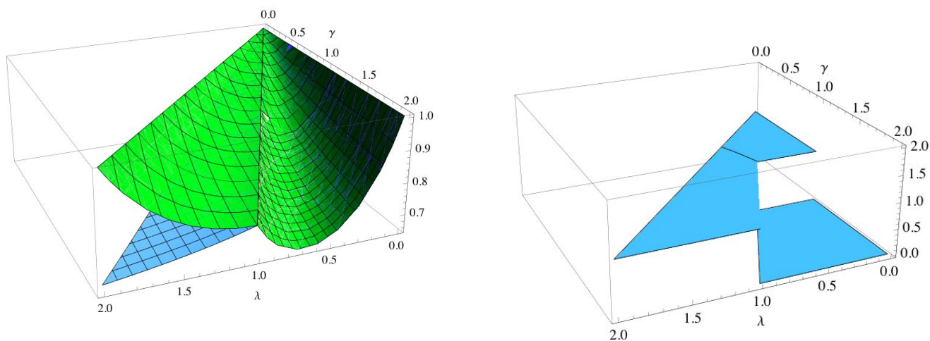
Figure 3: Probability of peace in the mediated vs. unmediated case, and region where mediation dominates
