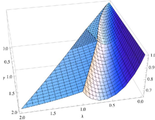
Figure 1: Probability of peace in the separating equilibrium
