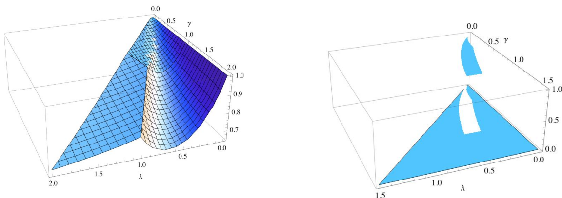
Figure 2: Welfare in the best (pure or mixed) equilibrium, and region where mixing occurs
