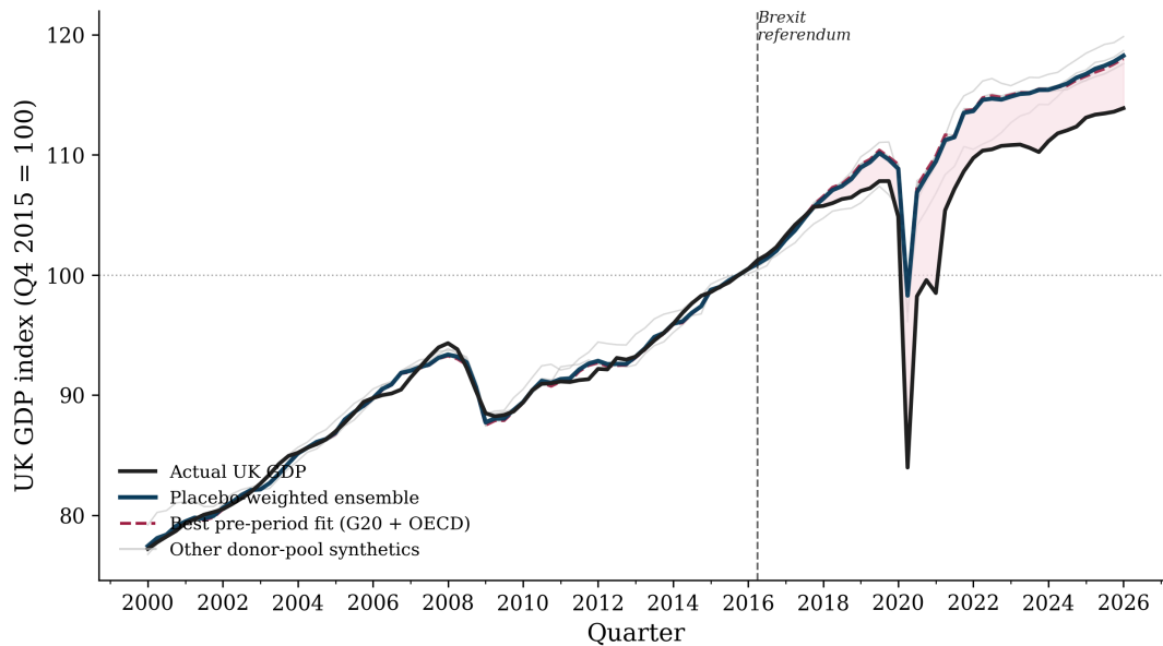
Figure 1: UK quarterly GDP: synthetic control estimates across donor pools, post-2016
