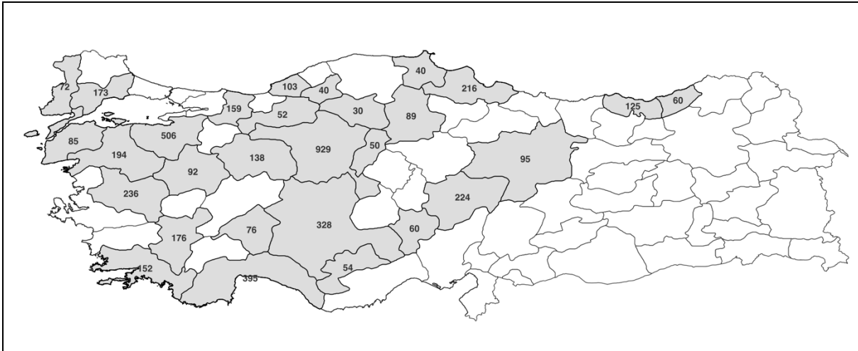
Figure II. Sampling Distribution
